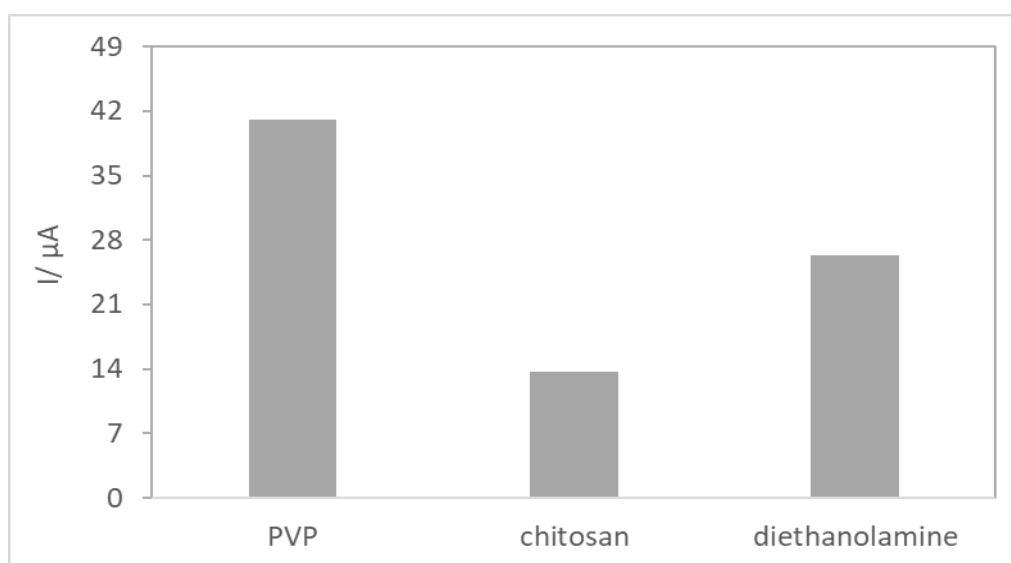
Figure 1. Currents obtained for carbon-printed electrodes containing \text{Fe}_3\text{O}_4@\text{Ag} core-shell coated with different compounds. In 300 \text{ mg L}^{-1} amoxicillin solution in 0.1 \text{ mol L}^{-1} phosphate buffer pH 7.0. Pulse amplitude was 25 \text{ mV} , at 50 \text{ mV s}^{-1} .
