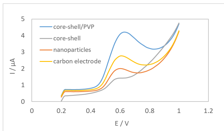
Figure 4. Differential Pulse Voltammograms of the \text{Fe}_3\text{O}_4 nanoparticles (A); \text{Fe}_3\text{O}_4@\text{Ag} core-shell nanostructure (B) \text{Fe}_3\text{O}_4@\text{Ag}/\text{PVP} nanocomposite (C) in 136 \mu\text{mol L}^{-1} amoxicillin solution in 0.1 \text{ mol L}^{-1} phosphate buffer pH 7.0 and \text{Fe}_3\text{O}_4@\text{Ag}/\text{PVP} nanocomposite in 0.1 \text{ mol L}^{-1} phosphate buffer pH 7. Pulse amplitude was 25 mV, at 50 \text{ mV s}^{-1} .
