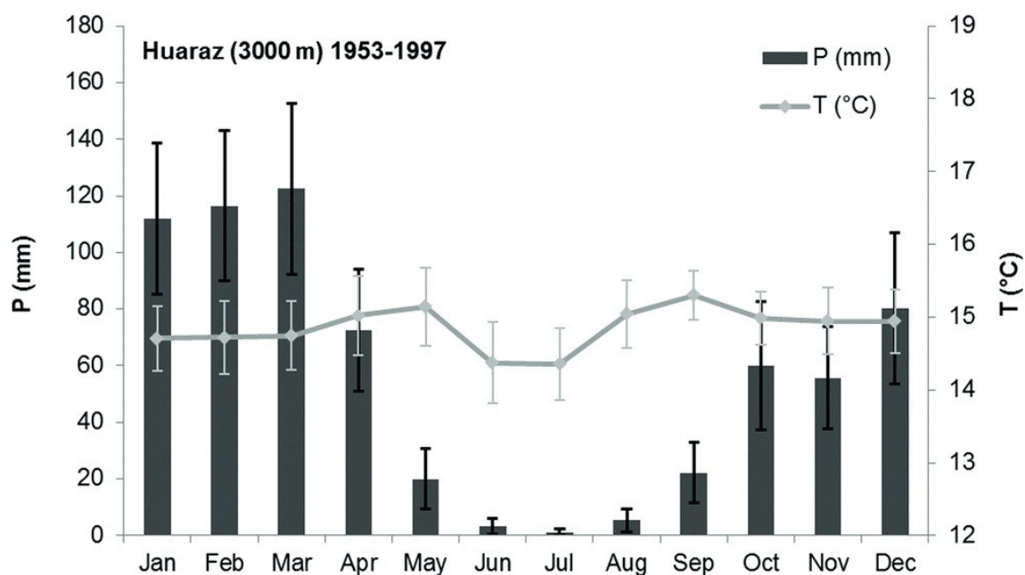
Figure 1 – Historical record averages for precipitation (P) and temperature (T) for Huaraz between 1953 and 1997.
