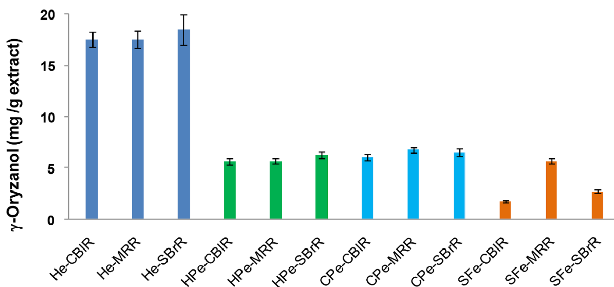
Figure 1. \gamma -oryzanol content in CBIR, SBrR, and MRR bran oil extracted by He, HPe, CPe, and SFe. The values were represented as mean \pm SD.
