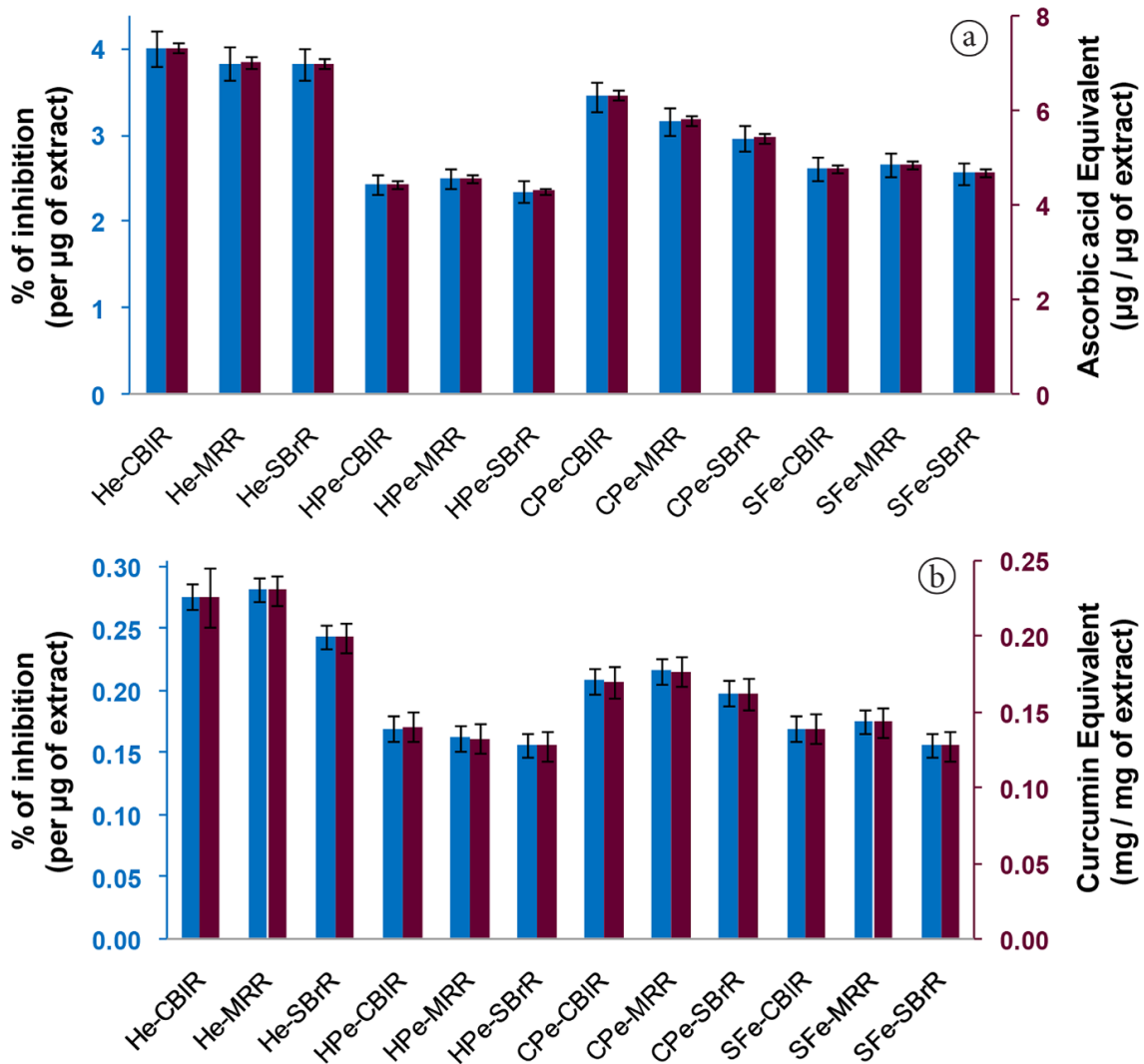
Figure 5. Superoxide (O 2 •- ) radical (a) and nitric oxide (NO • ) radical (b) scavenging activity of RBO extracts in comparison with its standard. The values were represented as mean ± SD.
