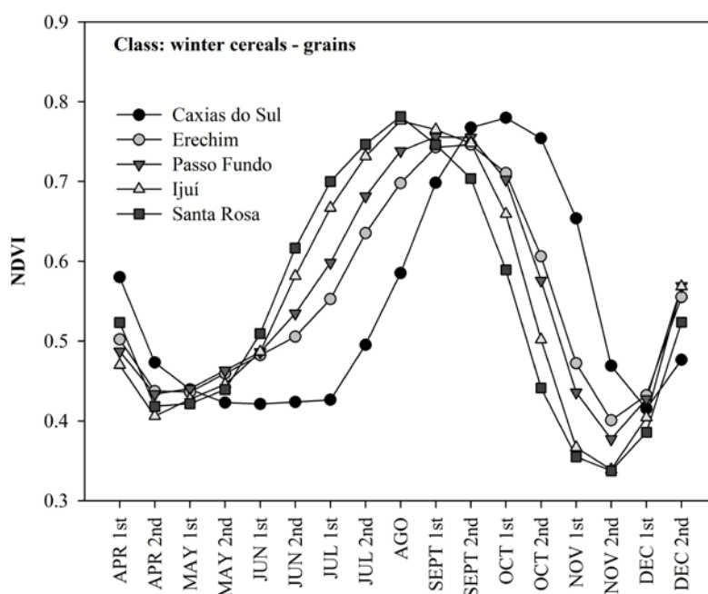
FIGURE 4. NDVI/MODIS average temporal profiles of class 2 (winter cereals for grain production), fortnights from April to December, in the Caxias do Sul, Erechim, Passo Fundo, Ijuí and Santa Rosa regions; average from 2000 to 2008.
