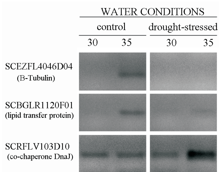
Figure S1 - Differential gene expression analyzed by RT-PCR in the sugarcane genotype RB72910 under simulated drought stress. Three genes ( \beta -tubulin, LTP and DnaJ) were amplified by PCR with 30 and 35 cycles and the amplification products were electrophoresed on 3% (w/v) agarose gels.
