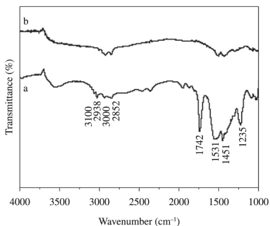
Figure 3. FT-IR spectra of \text{TiO}_2 nanoparticles a) before and b) after treatment under ozone flow for 1 h.
