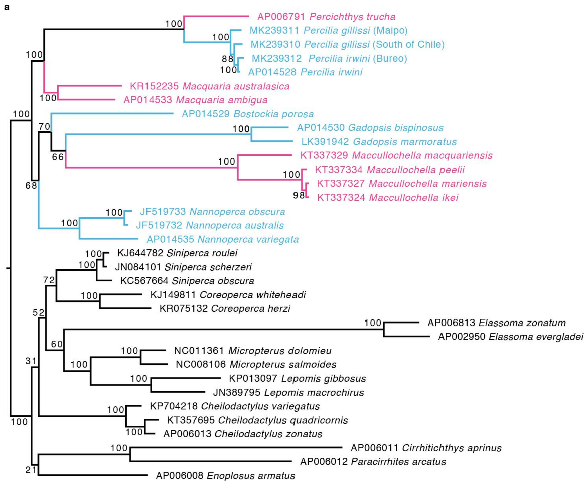
Figure S2. Mitogenomic maximum likelihood tree of Percichthyidae sensu Lavoué et al. (2014) and Betancur-R et al. (2017) considering newly assembled and available mitogenomic sequences. (a) Partitioned data matrix with three partitions (Mt1). (b) Partitioned data matrix with four partitions (Mt2). Numbers at nodes are bootstrap support [bs]. Representatives of Percichthyidae are shown in pink, representatives of Perciliidae are shown in light blue.
