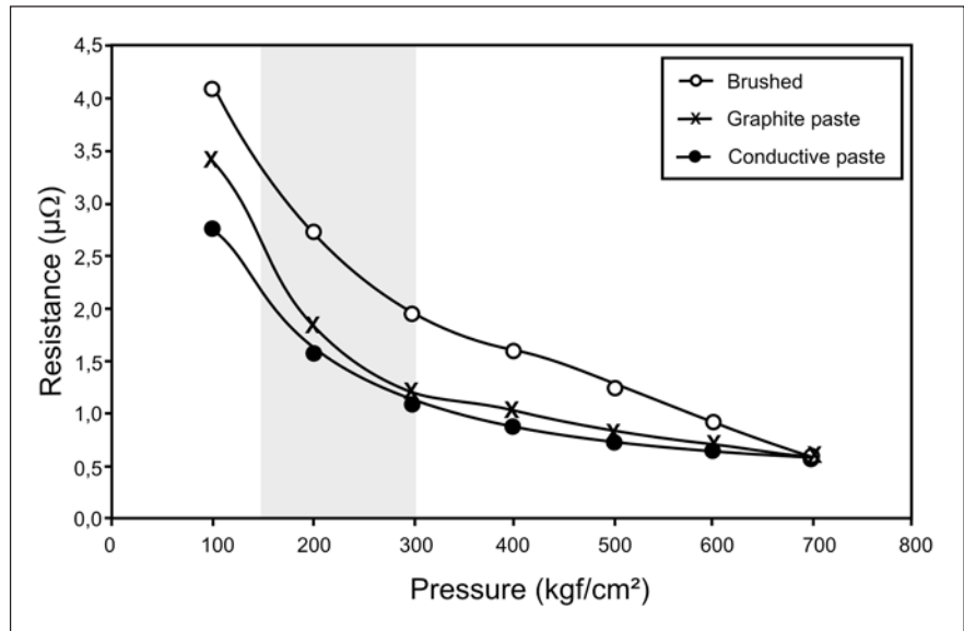
Figure 2 - Resistance of the Cu/Cu joint as a function of pressure, for the joints with simply brushed surfaces, and for the joints brushed and filled with either graphite paste or conductive paste. Dark area represents the usual range of pressures at the joint in industry.
