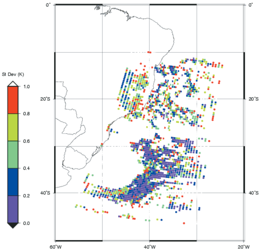
Figure 6 – Standard deviation estimates (test T4) for each area within a 3 \times 3 pixel from NOAA 15 image on February 23, 2000 at 10:02 UTC.
