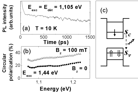
FIG. 1: (a) Intensity of the QD ground state PL for intradot strictly resonant excitation and detection at 1.105 eV. Note that the first decay (at t < 100 \text{ ps} ) is due to the laser backscattered light. (b) Circular polarization of the QD ground state luminescence for (●) B_z = 0 and (△) B_z = 100 \text{ mT} ; the excitation energy is 1.44 eV, i.e. in the wetting layer (c) Scheme of a positively charged exciton X^+ formed by a spin polarized electron and two holes with opposite spin angular momentum projection.
