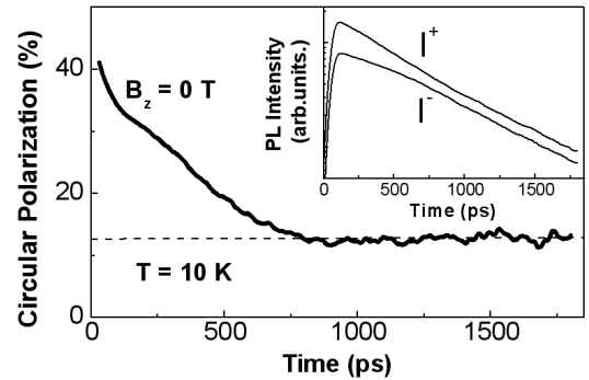
FIG. 2: Circular polarization dynamics of the QD luminescence after a circularly polarized \sigma^+ laser excitation; E_{\text{exc.}} = 1.44\text{eV} . Inset: photoluminescence intensity co-polarized I^+ and counter-polarized I^- with the laser (semi-logarithmic scale). The detection energy is centred at E_{\text{det.}} = 1.11\text{eV} .
