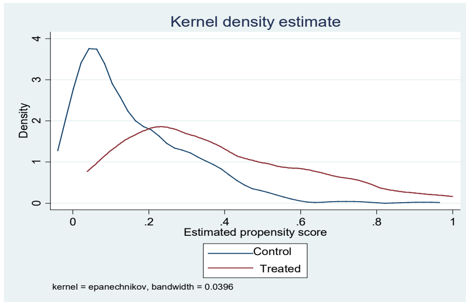
Figure 1- Kernel density estimate
