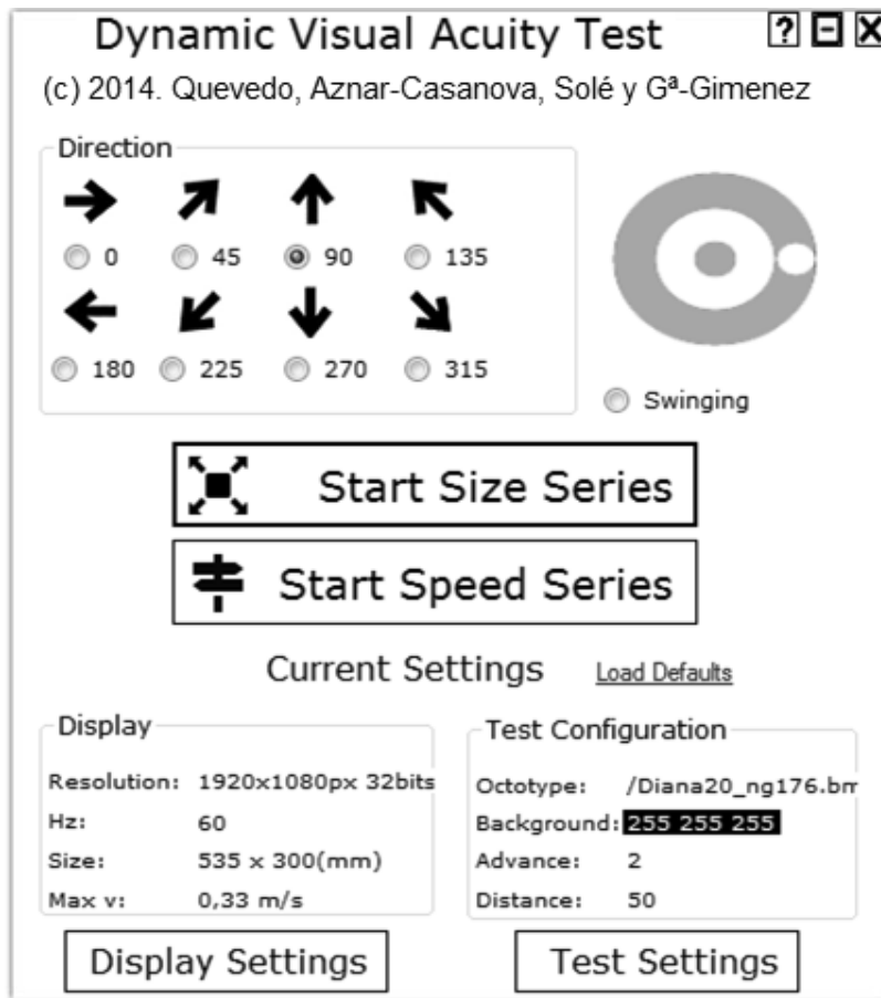
Figure 6. The DynVA is a computer software designed to assess DVA. The researcher can select the optotype to be presented in the two forms of the test: (a) Size Series; (b) Speed Series. In the Size series, the optotype size remains constant, while its speed decreases as it moves across the screen. Conversely, in the Speed series, the optotype speed remains constant while its size increases progressively as it moves across the screen. In both series, the trial ends when the subject presses the arrow key that matches the position of the band gap of the test card.
