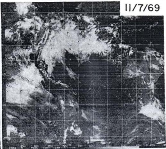
Composite satellite pictures (July 8 th. - July 11 th., 1969).
