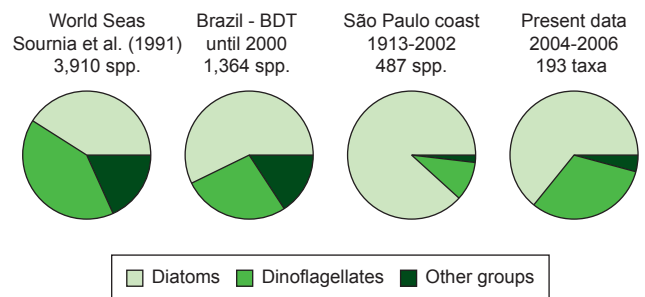
Figure 3. Relative contribution of the main taxonomic groups at different levels: worldwide (Sournia et al. 1991), Brazil (Banco de Dados Tropical - www.bdt.fat.org.br/workshop/costa), pre-existing data for the state of São Paulo (references in Table 1), and primary data for the state of São Paulo.
