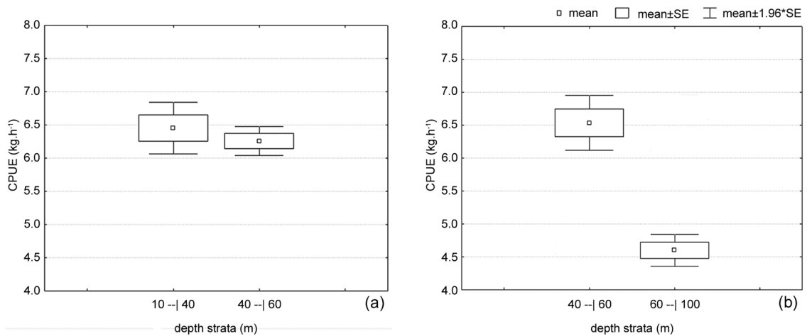
Figure 3. CPUE (kg.h -1 ) for southern brown shrimp for depth strata in the Amazon (a) and the Amapá coast (b) sites (SE: standard error).
