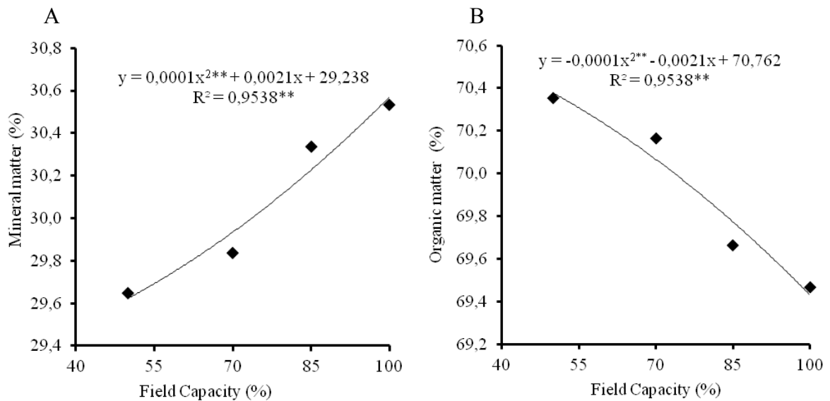
Figure 5. Regression equations relating Mineral Matter (MM) (A) and Organic Matter (OM) (B) of saltbush irrigated with waste from desalination differing in soil moisture level.
