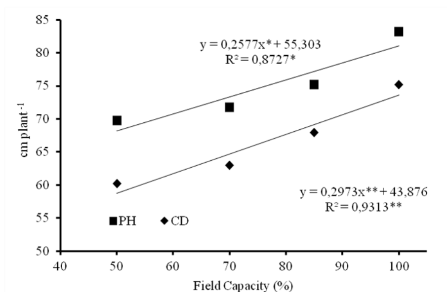
Figure 1. Linear regression equations relating plant height (PH) and crown diameter (CD) of saltbush ( Atriplex nummularia L.) irrigated with waste from desalination differing in soil moisture level.
