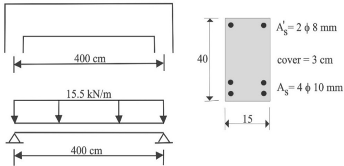
Figure 7. Reference beam.
