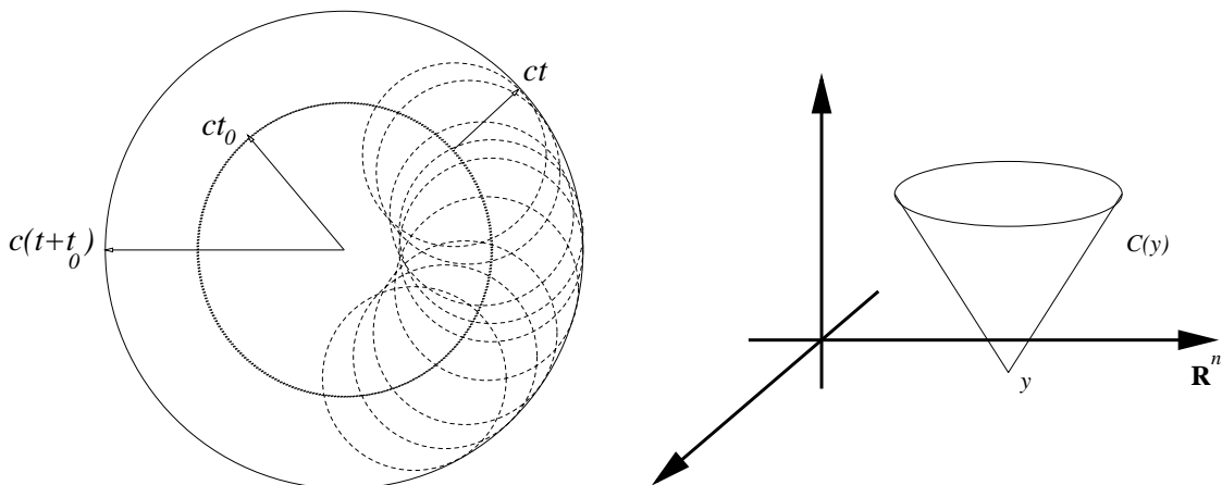
Fig. 1 – Huygens’ construction of a wave front from the previous one (left). Forward light cone with vertex in y (right).
