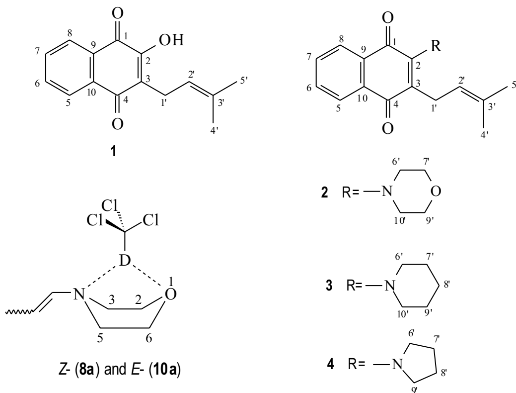
Fig. 1 – Structures lapachol ( 1 ), lapachol derivatives ( 2,3,4 ) and model compounds 8 and 10 involved in intermolecular hydrogen bond with \text{CDCl}_3 ( 8a and 10a ).
