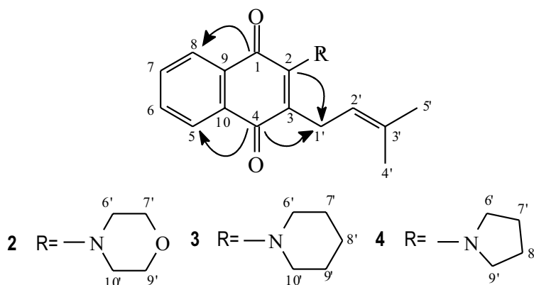
Fig. 3 – Selected HMBC correlations for compounds 1-4 .
