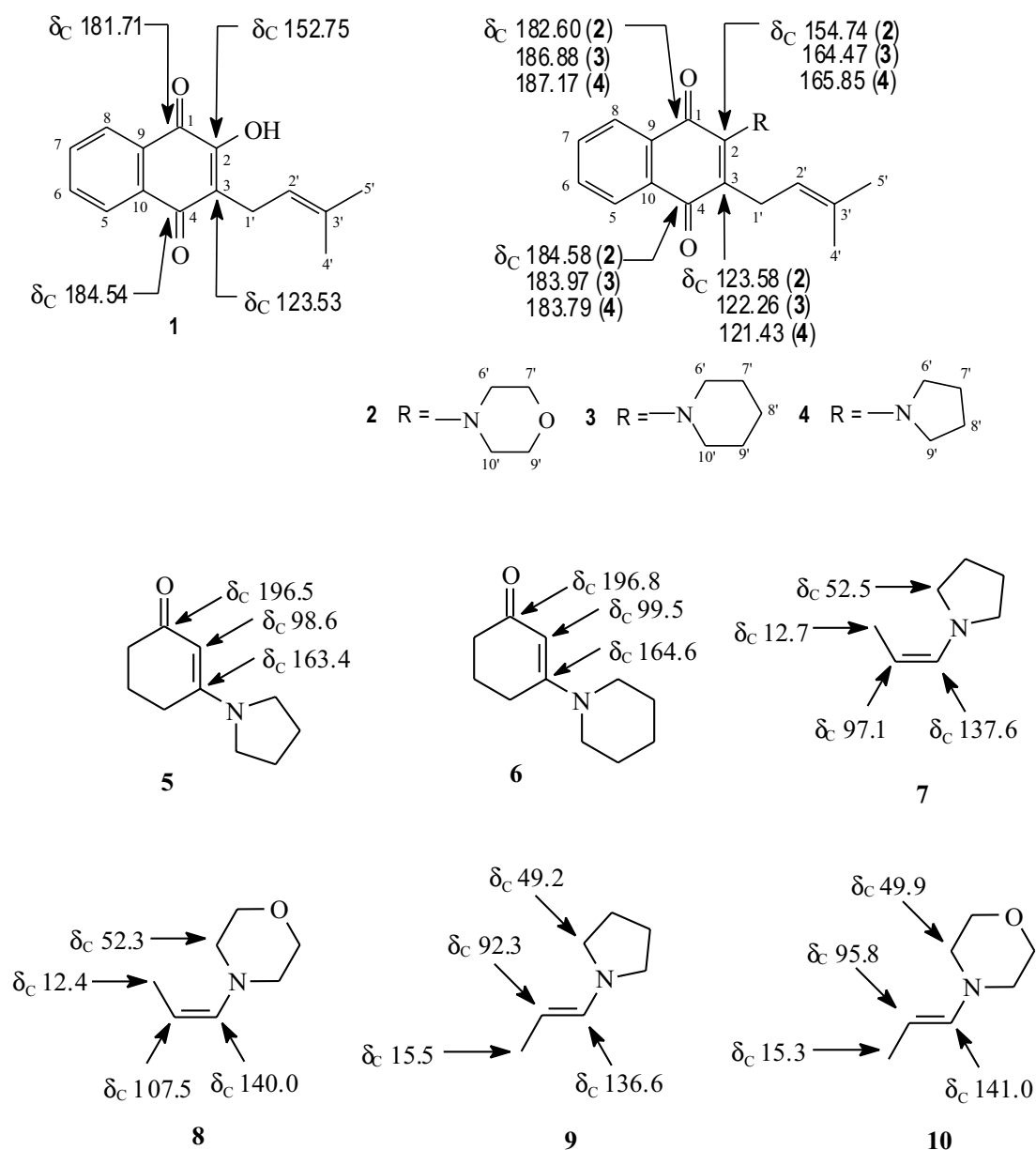
Fig. 4 – ^{13}\text{C} NMR spectral data of enamine derivatives 2-4 and model compounds 5-10 described in the literature (Giasuddin et al. 1978, Breitmaier and Voelter 1987).
