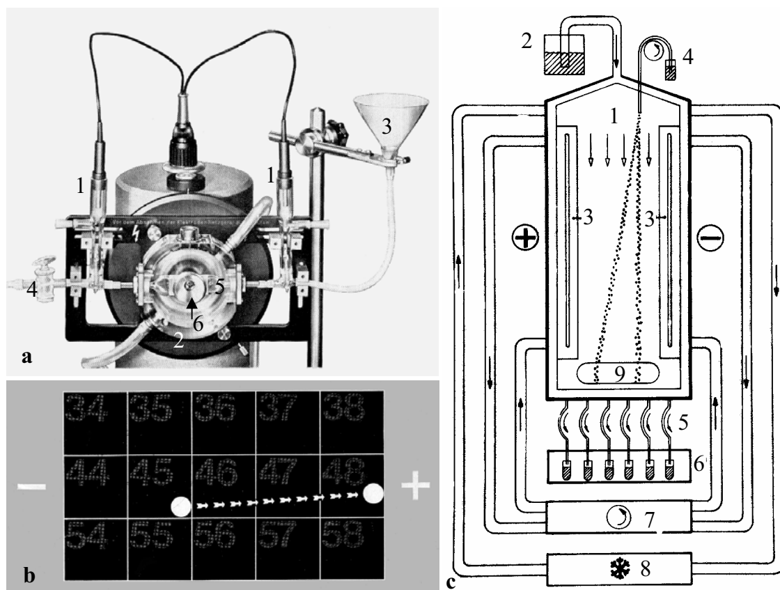
Fig. 3 – Principle and construction diagrams of microelectrophoresis (a-b) and free-flow electrophoresis. Fig. 3a – 1) Electrode compartment in electrical contact with the measuring chamber via a membrane; 2) Temperature controlled chamber connected to the circulating thermostat; 3) Funnel-cells in normal saline solution were introduced into the measuring chamber through plastic tubes. The liquid stream is controlled by a cock (4); 5) Measuring chamber; 6) Viewing window-place where the front lens of the microscope objective had to be connected to the temperature-controlled chamber. Fig. 3b – One of the focusing eyepieces of the light microscope contains a special reticule which serves as micrometer. The time it takes a cell edge to pass two or more whole micrometer intervals is measured with the aid of a stopwatch. Fig. 3c – 1) Separation chamber; 2) Chamber buffer; 3) Electrode compartment in electrical contact with the separation area via a membrane; 4) Sample pump; 5) Multitube pump; 6) Cooled fraction container with vials for sample collection; 7) Electrode buffer circulation; 8) Electronically regulated cooling system. 9) Optical window for analytical measurements.
