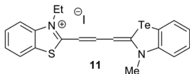
Fig. 9 – Molecular structure of the thiatelluracarboxyanine iodide 11 .
