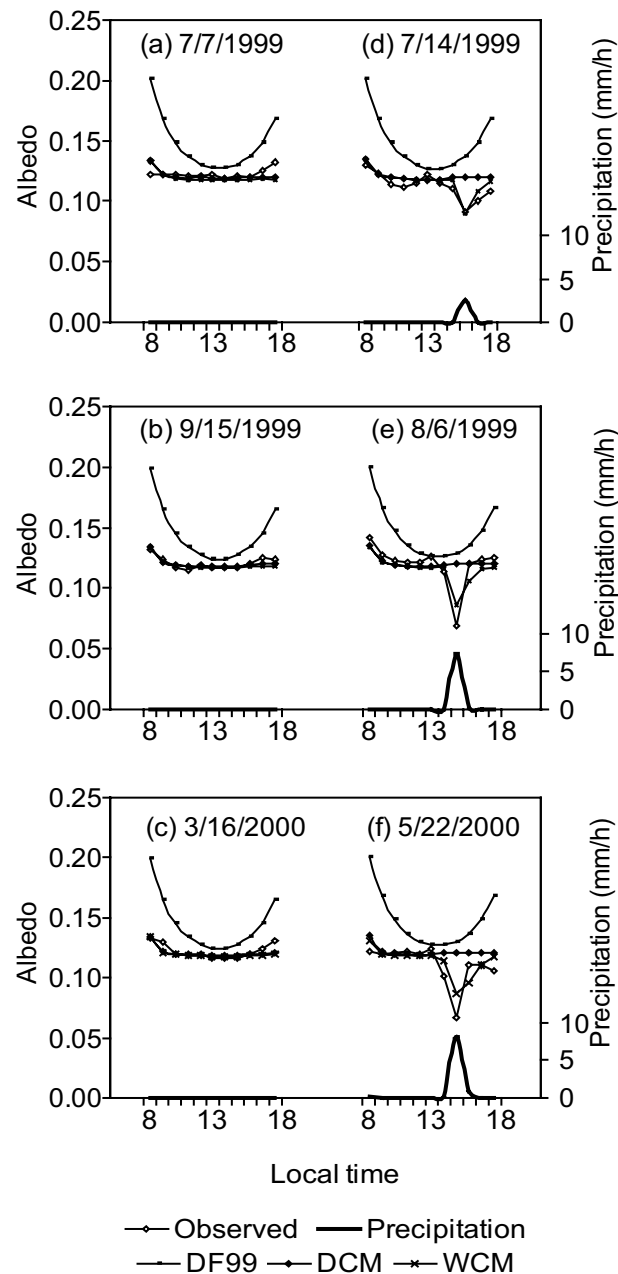
Fig. 2 – Diurnal variation of the simulated and observed surface albedo in the Cuieiras Reserve for the selected days.
