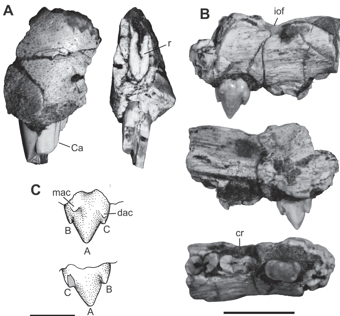
Fig. 3 - Holotype (MMACR-PV-003-T) of Botucaratherium belarminoi gen. nov. et sp. nov. A: Fragment of left maxilla with portion of canine in lateral and posterior views. B: Fragment of left maxilla with postcanine in lateral, medial and ventral views. C: Detail of upper postcanine in labial (lateral) and lingual (medial) views. Scale bars equals 5 mm in A and B and 2 mm in C. Gray areas indicate broken surfaces. Abbreviations: A-C , refers to name of cusps; Ca , upper canine; cr , constricted root; dac , distal accessory cusplule; iof , ventral edge of the infraorbital foramen; mac , mesial accessory cusplule; r , root.
