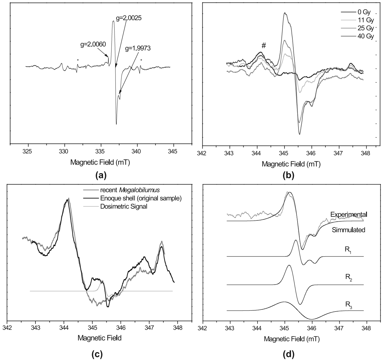
Figure 2 - ESR X-Band spectrum of the shell recorded in the Jeol spectrometer (USP). (a) Spectrum of the aliquot irradiated with a dose of 700 Gy recorded together with the secondary standard of Mn^{2+} , showing the main radicals present in the g \sim 2 region. The * indicates the 3 rd and 4 th Mn^{2+} lines. Modulation amplitude = 0.05mT, microwave power = 1 mW, scan width = 20 mT, total of 10 scans. (b) Spectrum of irradiated aliquots centered in the g \sim 2 region, showing intensification of the CO_2^- signal and the SO_2^- radical region (#) (c) Spectrum of the original sample (0 Gy) after storage of 1000 scans (black line), showing the dosimetric signal superposed by the spectrum simulation of the CO_2^- radical (light gray line) and the spectrum of recent Megalobilumus . (d) ESR spectrum deconvolution showing the main paramagnetic centers created by irradiation. R_1 is the axial CO_2^- radical with g_{\perp} = 2.0025 and g_{\parallel} = 1.9973 , and R_2 is the isotropic CO_2^- radical with g = 2.0007 . R_3 is an unknown radical.
