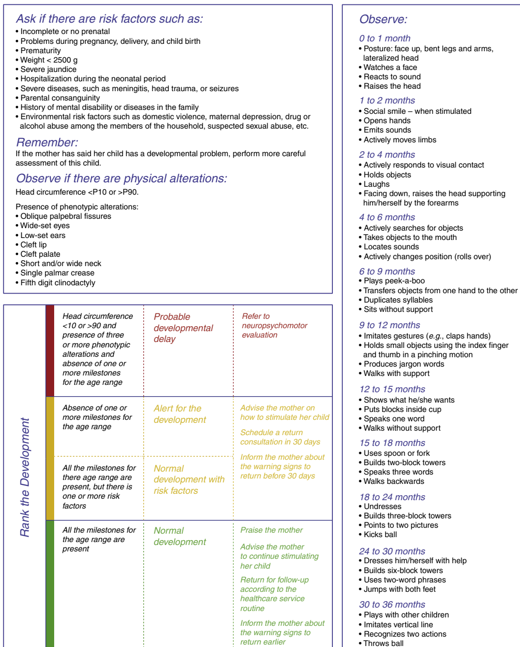
Figure 1 Surveillance algorithm.
