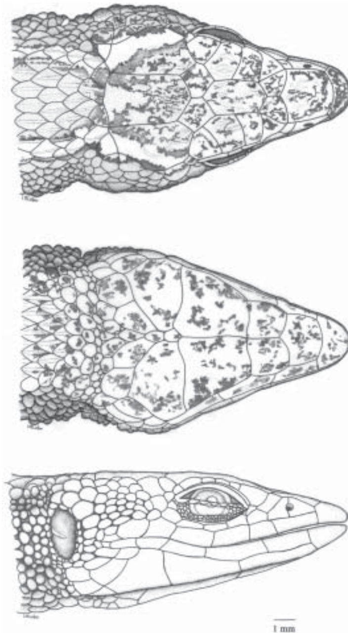
Figure 1. Dorsal, ventral, and lateral view of head of the holotype of Leposoma puk from Una, state of Bahia, Brazil (MZUSP 87959).
