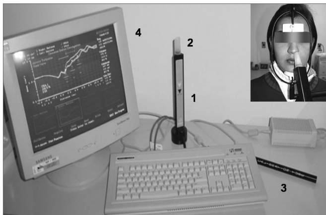
Figure 1. Acoustic rhinometer (Eccovision, Hood Laboratories): instrumentation to check nasal cavity cross-sectional areas; 1= sound tube; 2= nasal adapter; 3= calibration tube 4= computer monitor showing a rhinogram. See patient in position for data acquisition.
