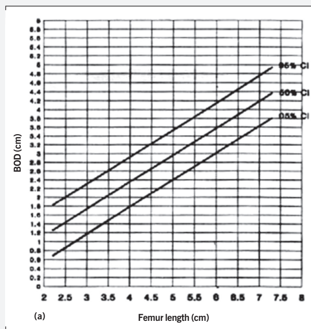
Fig. 1 - Normality curve of femur length X BOD.
