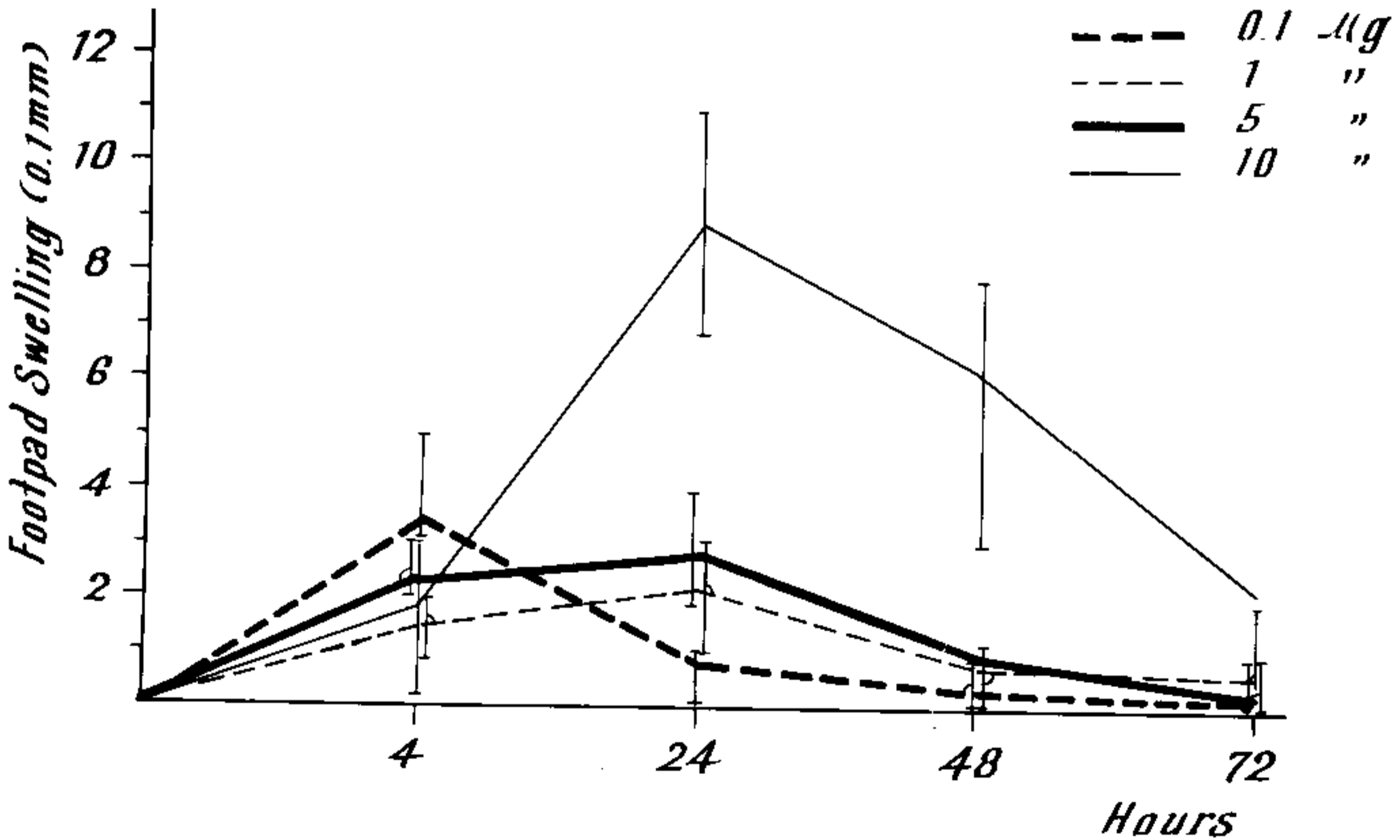
Fig. 3 - Levels of DTH measured in BCG-immune-mice sensitized with 10 \mu g of flagellar fraction and elicited with different protein content doses of flagellar fraction from Trypanosoma cruzi epimastigotes as expressed in the figure. Mean of five mice \pm standard deviation.
