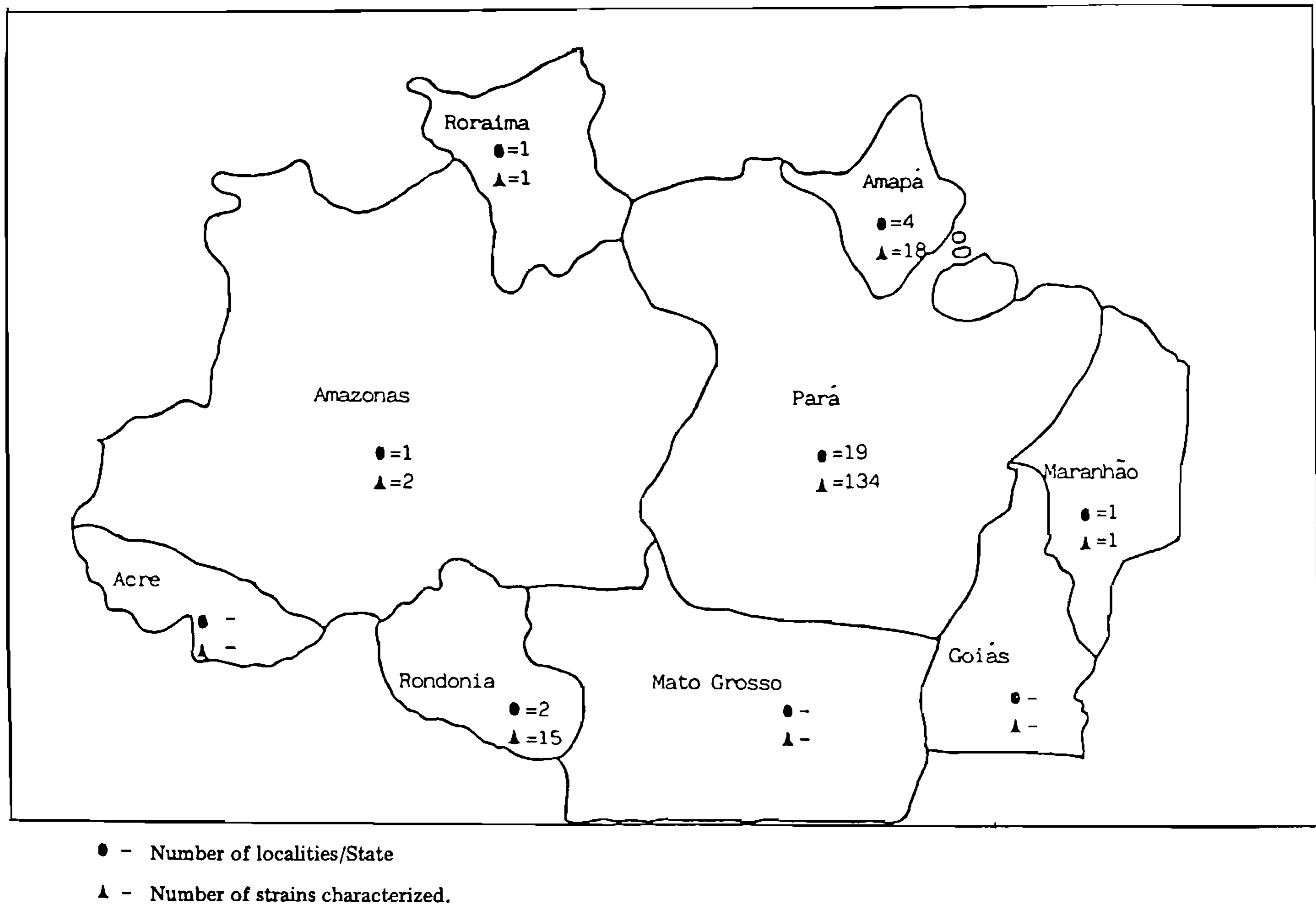
Fig. 1: Brazilian Amazon Region: collection of samples.
