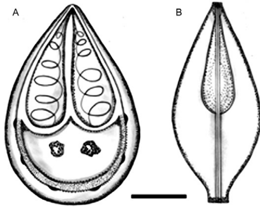
Fig. 5: schematic representation of mature spores of Myxobolus oliveirai sp. nov. A: frontal view; B: lateral view. Bar = 3 μm.
