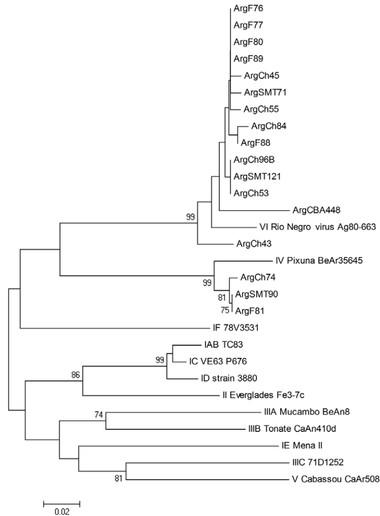
Fig. 2: dendrogram constructed with Neighbour joining method and p-distance parameter included positive sample ArgCba448, prototype Venezuelan equine encephalitis complex viruses and previous Argentinean isolates, indicated by ArgCh (isolates from the province of Chaco), ArgF (isolates from the province of Formosa) and ArgSMT (isolates from the province of Tucumán) (GenBank accessions EU649784, EU658924, EU658925, EU848531, EU848532, EU848534, EU848536, FJ002856, FJ002857, GQ885141, GU002046, HM804026 and HM991260). The number of replicate trees in which the associated taxa clustered together in the bootstrap test (1,000 replicates) is shown next to the branches.
