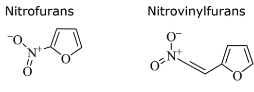
Fig. 1: structural difference between nitrofurans (nitrogen bonded to the furan ring) and nitrovinylfurans (nitrogen bonded to the side vinylic chain).
