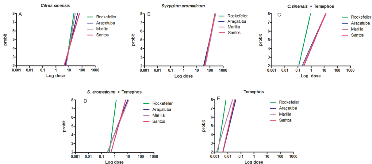
Fig. 1: dose-response curves created using bioassay data after exposure to the essential oils of Citrus sinensis (A) and Syzygium aromaticum (B), temephos combinations (C-D) and temephos alone (E).
