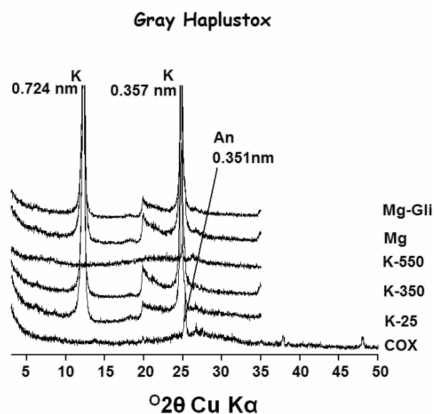
Figure 2. X ray diffractograms of the deferrified clay fraction and oxide concentrations in the Bw 2 horizon of the "Gray Haplustox" ("LAC"). K: Kaolinite and An: Anatase.
