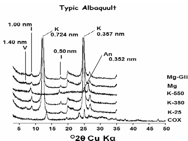
Figure 1. X ray diffractograms of the deferrified clay fraction and oxide concentrations in the Btg 2 horizon of the typical Albaquilt (GXbd). K: Kaolinite, I: Illite, An: Anatase, and V: Vermiculite (traces).
