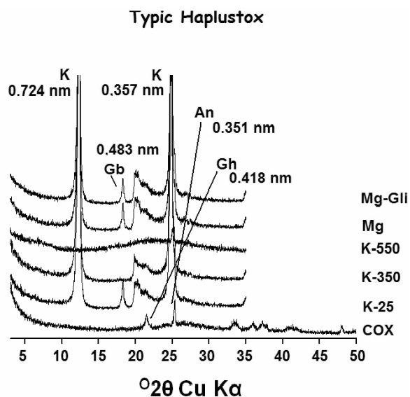
Figure 4. X ray diffractograms of the deferrified clay fraction and oxide concentrations in the Bw 2 horizon of the Red Yellow Latosol (LVA). K: Kaolinite, Gb: Gibbsite, Gh: Goethite, and An: Anatase.
