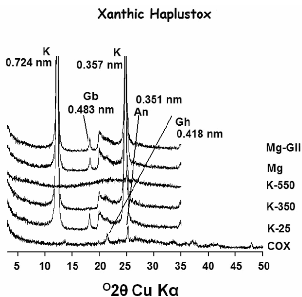
Figure 3. X ray diffractograms of the deferrified clay fraction of the Bw horizon of the Xanthic Haplustox (LA). K: Kaolinite, Gb: Gibbsite, Gh: Goethite, and An: Anatase.
