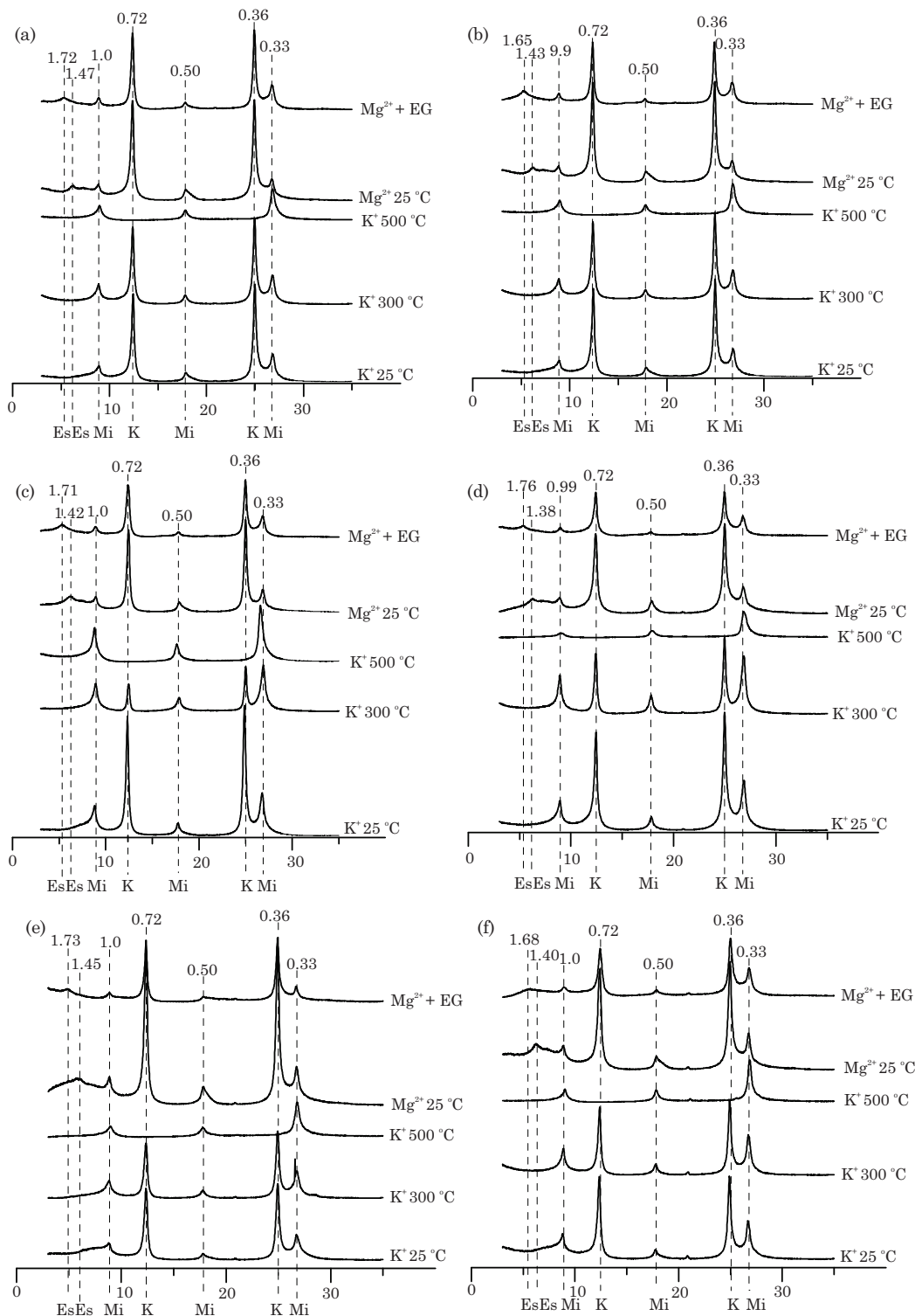
Figure 6. Diffractograms ( ^{\circ}2\theta CuK \alpha ) of total clay in horizons after (a, c, e) and before (b, d, f) the avulsion process in AP1: (a) 30-75 cm - post, (b) 145-200 cm - pre; AP4: (c) 30-45 cm - post, (d) 150-190 cm - pre; and AP10: (e) 105-150 cm - post. K=Kaolinite, Mi=Mica, Es=Smectite.
