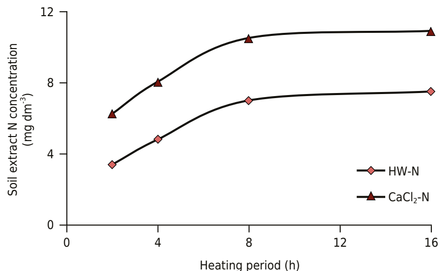
Figure 1. Average N concentrations in soil extracts of 17 soil samples using hot water (HW-N) and a hot solution of 0.01 mol L -1 CaCl 2 (CaCl 2 -N) under increasing heating periods (2, 4, 8, and 16 h heating periods).
