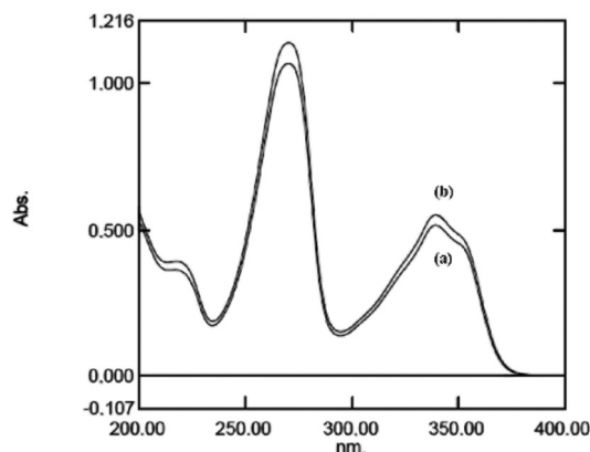
Figure 2. UV-absorption spectra of 12.0 \mu\text{g mL}^{-1} concentration of GFM commercial sample (a) and GFM RS solutions (b) in methanol
