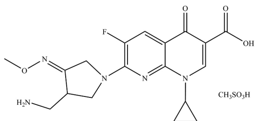
Figure 1. Chemical structure of GFM
