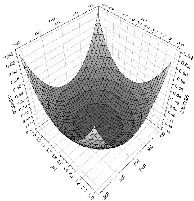
Figure 1. Response surface of COD removal of Zn-EDTA by the CAT-driven Fenton reaction, as a function of Fe(III) \mu\text{M} and pH at 25 °C, 2 h and CAT = 50 \mu\text{M}
