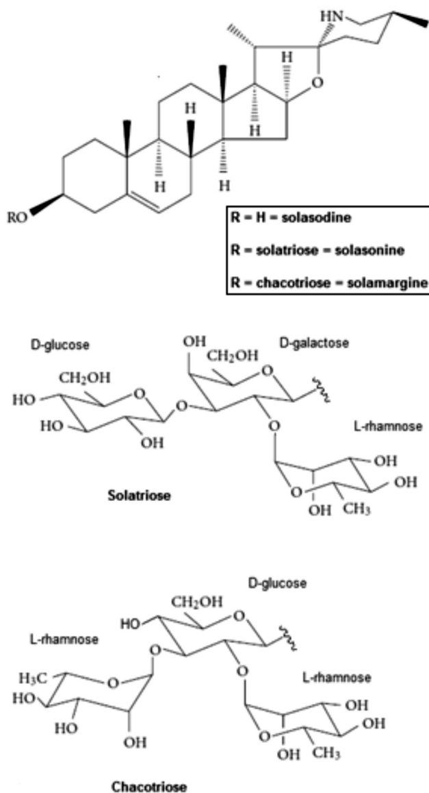
Figure 1. Chemical structures of Solanum lycocarpum glycoalkaloids: solasonine (SN) and solamargine (SM), and its aglycone solasodine
