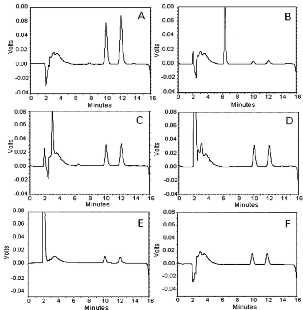
Figure 2. HPLC-UV chromatographic profiles of standards of solasonine (SN) and solamargine (SM) (A), topical formulation (B), samples spiked with alkaloidic extract (AE): stratum corneum (SC) (C), epidermis plus dermis [EP + D] (D), receptor solution (RS) (E), and AE of Solanum lycocarpum (F)
