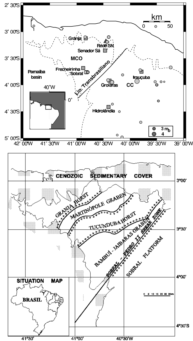
Figure 2 – Simplified maps of NW Ceará; a. Map showing the two main domains in NW Ceará. The Medium Coreáú Domain = MCO, the Ceará Central Domain = CC and Transbrasiliano lineament. The dashed line is the limit of the sedimentary basins. Circles are epicenters recorded by the UFRN network. Triangles indicate seismic stations. b. Figure showing the location of the Bambuí-Jaibaras, and Martinópole grabens separated by the Tucunduba horst (Figure taken from Sial et al. , 2000 – p. 550, Fig. 9).
