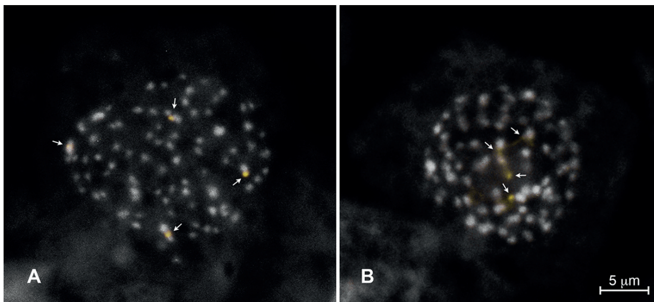
Figure 4. Mitotic metaphases of Cyperus ligularis and C. odoratus stained with CMA and DAPI. Cell of C. ligularis with 2n = 82 . A. Cell of C. odoratus with 2n = 72 . B. Arrows indicate satellite regions with bands CMA + /DAPI + .
