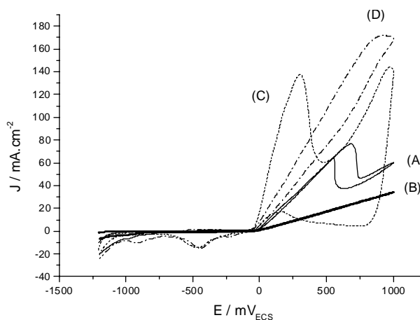
Figure 5. Influence of acetate concentration on voltammograms obtained with the alloys disc electrodes, between E_{sc} = -1.0 \text{ V} and E_{sa} = 1.0 \text{ V} at 0.001 \text{ V s}^{-1} , under static conditions: (A) Cu37Zn in 0.1 \text{ mol L}^{-1} Ac solution, (B) Cu37Zn in 1 \text{ mol L}^{-1} Ac solution, (C) Cu39Zn3Pb in 0.1 \text{ mol L}^{-1} Ac solution and (D) Cu39Zn3Pb in 1 \text{ mol L}^{-1} Ac solution.
