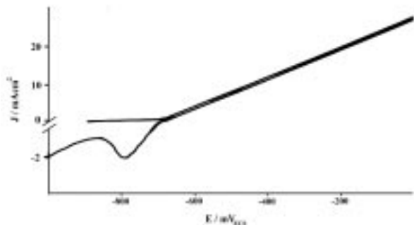
Figure 4. Voltammogram obtained with a Zn disc electrode in 0.1 \text{ mol L}^{-1} Ac solution, between E_{sc} = -1.0 \text{ V} and E_{sa} = 1.0 \text{ V} at 0.001 \text{ V s}^{-1} and under static conditions.
