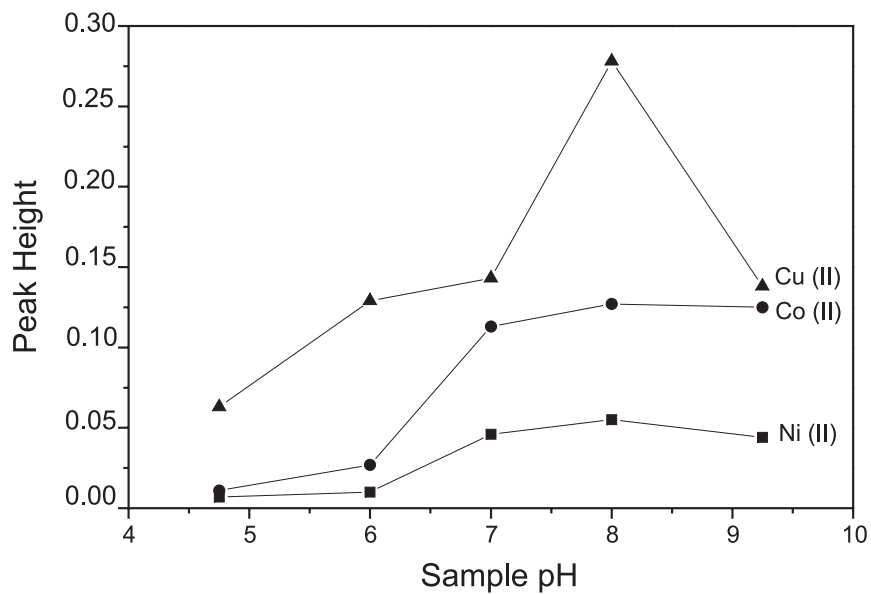
Figure 3. Effect of pH on the preconcentration of Cu, Co and Ni.
