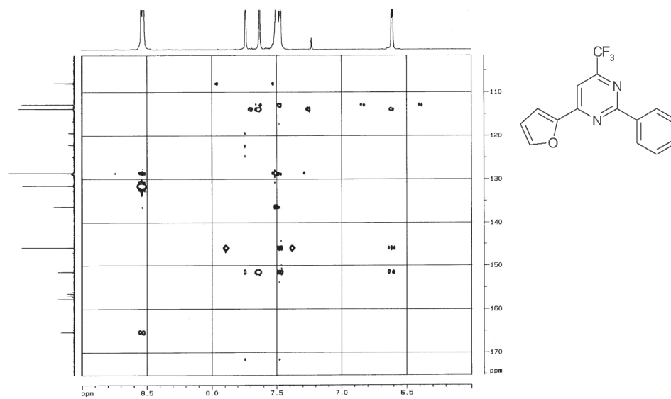
Figure S11. HMBC spectrum of the 6-(2-furyl)-2-phenyl-4-trifluoromethylpyrimidine 3b, CDCl 3 .
