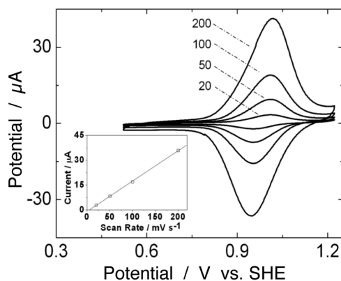
Figure 7. Cyclic voltammograms of a modified glassy carbon electrode containing three [\text{CuTRuPyPz}]^{4+}/[\text{CuTSPc}]^{4-} bilayers, surface coverage \Gamma = 1.86 \times 10^{-10} \text{ mol cm}^{-2} in 0.5 \text{ mol dm}^{-3} \text{ NaNO}_3 , pH 4.5 aqueous solution. Inset: plot of the peak current intensities as a function of the scan rate.
