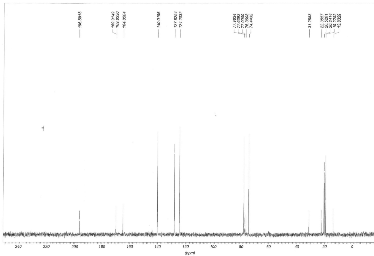
Figure S1. 13 C NMR (50 MHz, CDCl 3 ) Spectrum of the terrein ethyl derivative 2.
