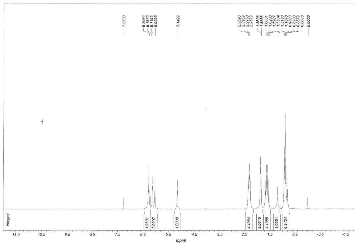
Figure S5. ^1\text{H} NMR (200 MHz, \text{CDCl}_3 ) Spectrum of the terrein butyl derivative 3 .
