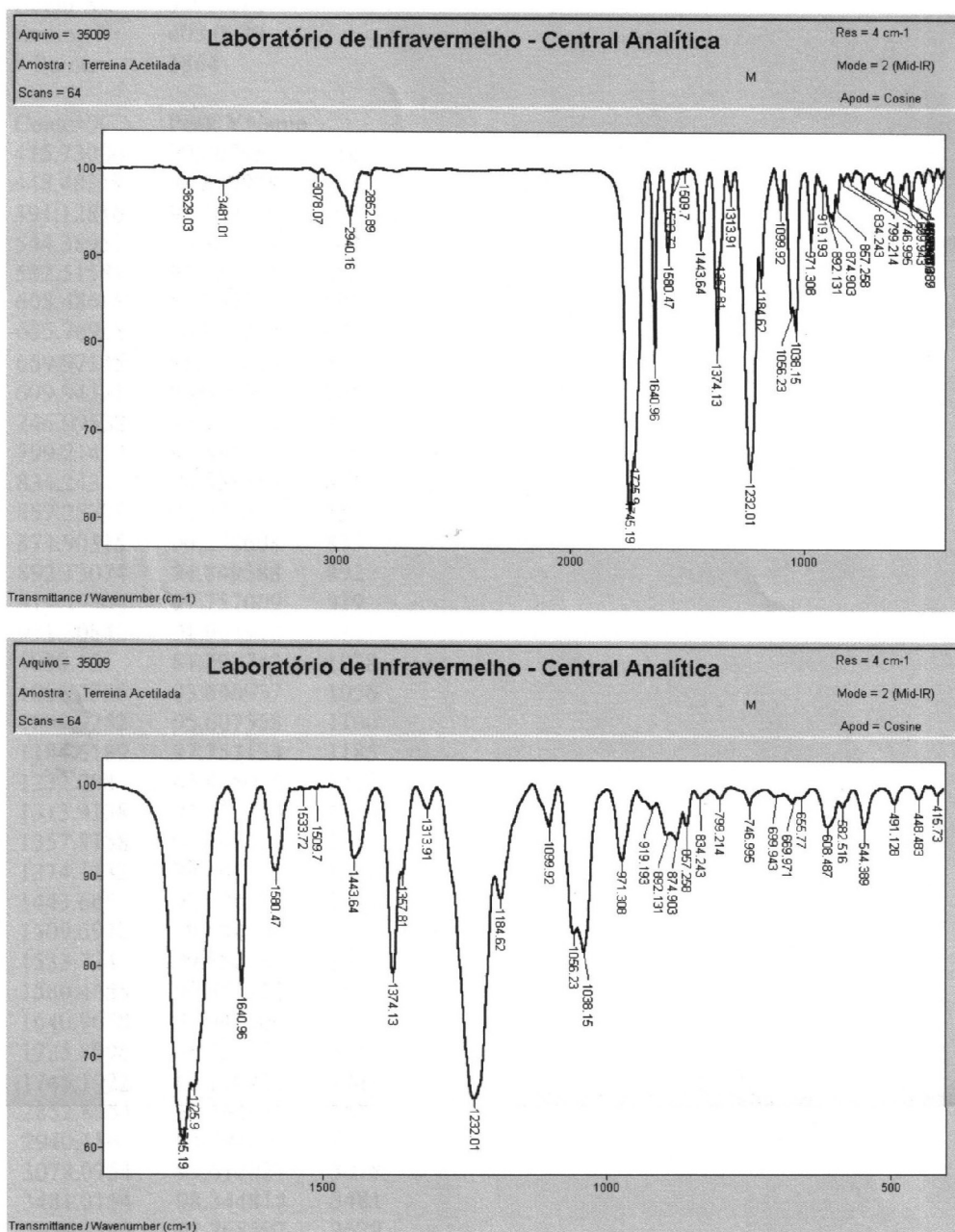
Figure S6. IR Spectrum of the terrein butyl derivative 3.
