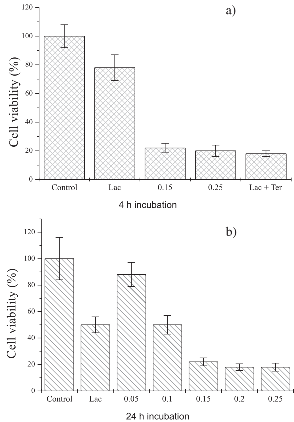
Figure 2. Cellular viability evaluation. Human lung tumoral cells were incubated: (A) 4 h and (B) 24 h in the presence of terrein and lactacystin. Lactacystin concentration was 5 \mu M and terrein concentrations shown were in the mM range.
