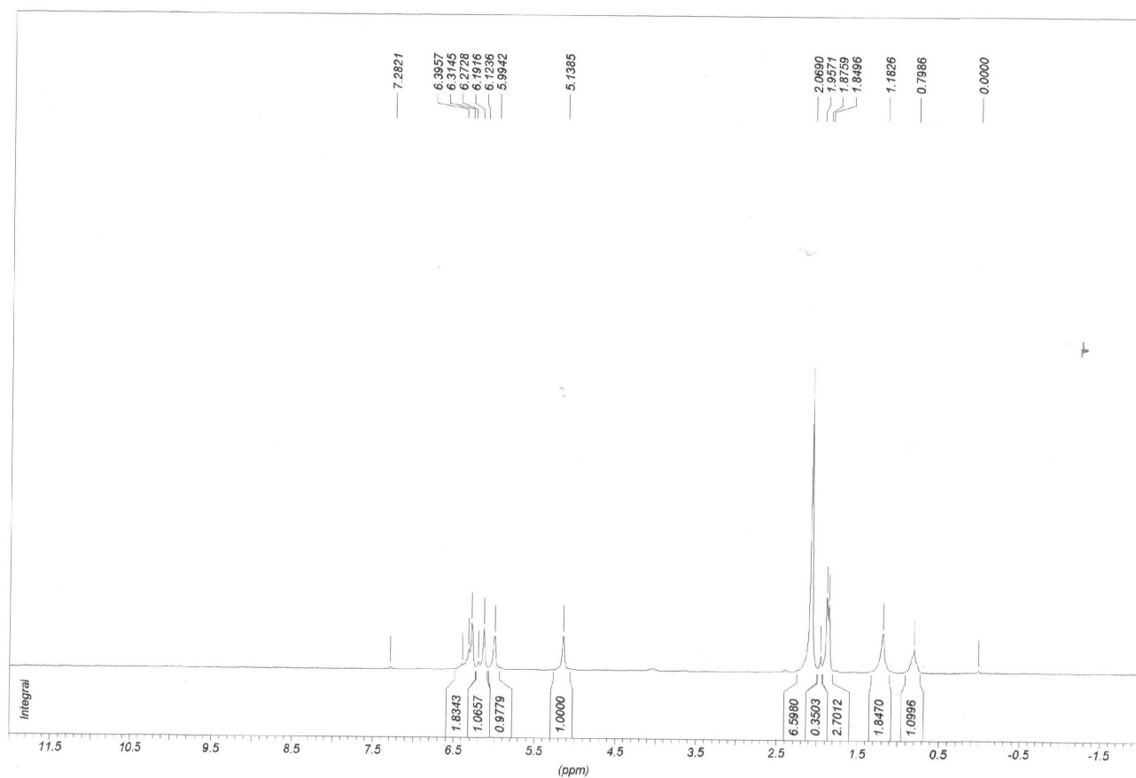
Figure S2. 1 H NMR (200 MHz, CDCl 3 ) Spectrum of the terrein ethyl derivative 2.
