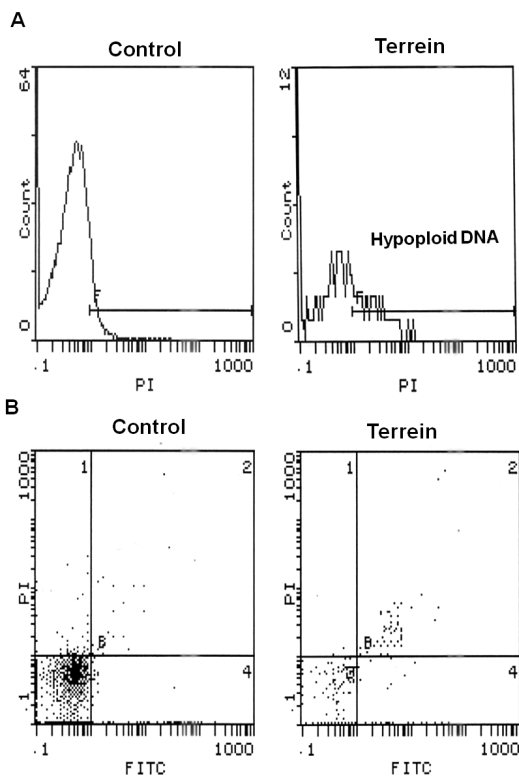
Figure 3. Flow fluorocytometry analysis of human lung tumoral cells incubated with terrein. (A) Cellular DNA labeling with propidium iodide. Cells after incubation (2 h) in the presence of 0.3 mM terrein were treated with 0.1% Triton and incubated with PI as described in Materials and Methods, followed by flow cytometry analysis. Control, representative of control samples, shows typical peak of PI fluorescence whereas terrein panel, representative of cellular samples incubated with 0.3 mM terrein for 2 h, shows decreased fluorescence and the presence of hypoploid DNA represented by the population of cells with lower fluorescence. (B) Cells after 4 h incubation with 0.3 mM terrein were incubated with Annexin V-FITC and PI, as described in Materials and Methods and analyzed by flow cytometry. As depicted, Control sample exhibit a homogeneous population of cells neither labeled with PI nor Annexin V-FITC. Terrein sample shows a representative double-labeled population of cells, as depicted in the top right quarter. Those cells are representative of the late onset of the apoptotic process.
