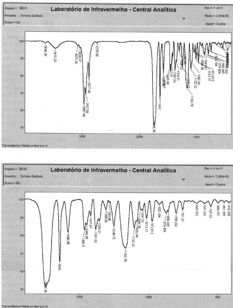
Figure S3. IR Spectrum of the terrein ethyl derivative 2.
