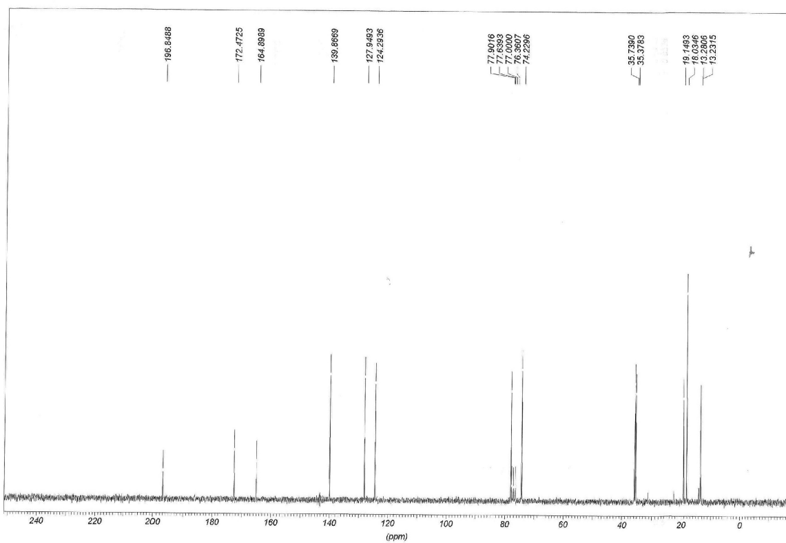
Figure S4. ^{13}\text{C} NMR (50 MHz, \text{CDCl}_3 ) Spectrum of the terrein butyl derivative 3 .
