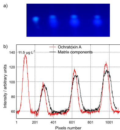
Figure 3. (a) HPTLC image of OTA with 11.5 \mu\text{g L}^{-1} of OTA standard solution and 5, 8 and 10 \mu\text{L} of sample extract without \text{NaHCO}_3 treatment. (b) Chromatogram constructed from HPTLC plate image by Image J software showing matrix components interfering in OTA quantification.
