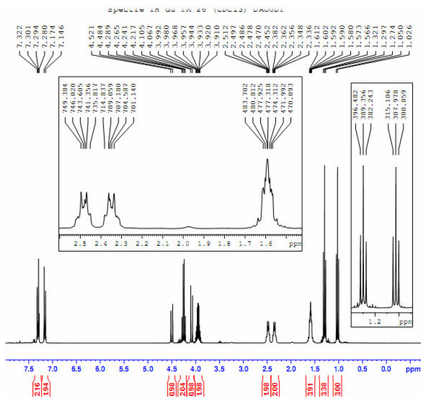
Figure S11. 1 H NMR (300 MHz) spectrum of compound 9 in CDCl 3 .
