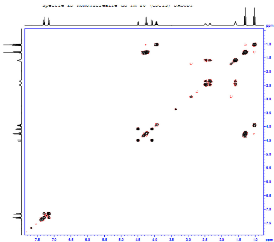
Figure S13. COSY of compound 9 in CDCl 3 .
