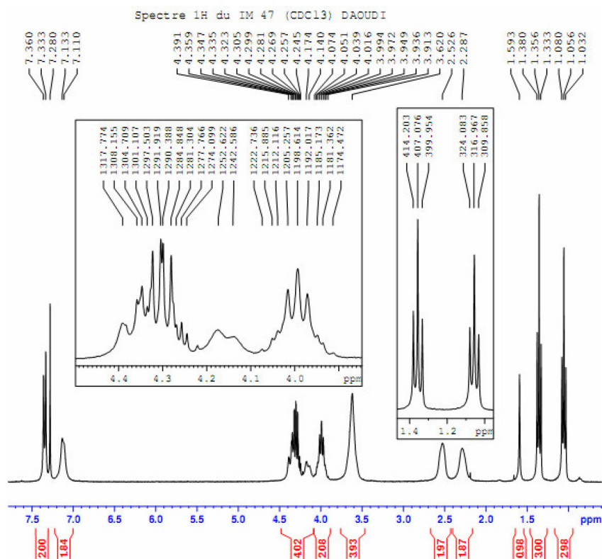
Figure S6. 1 H NMR (300 MHz) spectrum of compound 7 in CDCl 3 .
