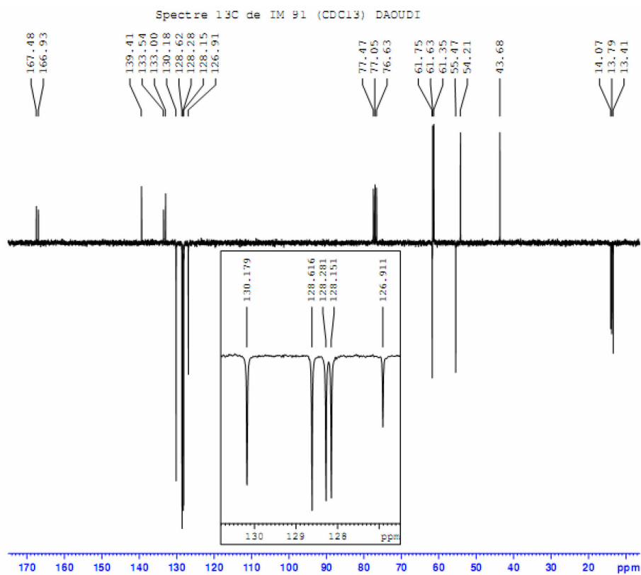
Figure S24. 13 C NMR (75.5 MHz) spectrum of compound 12 in CDCl 3 .
