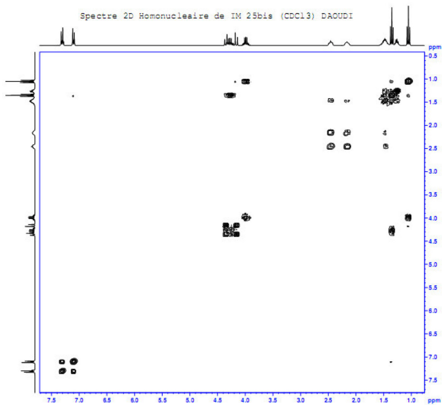
Figure S21. COSY of compound 11 in \text{CDCl}_3 .
