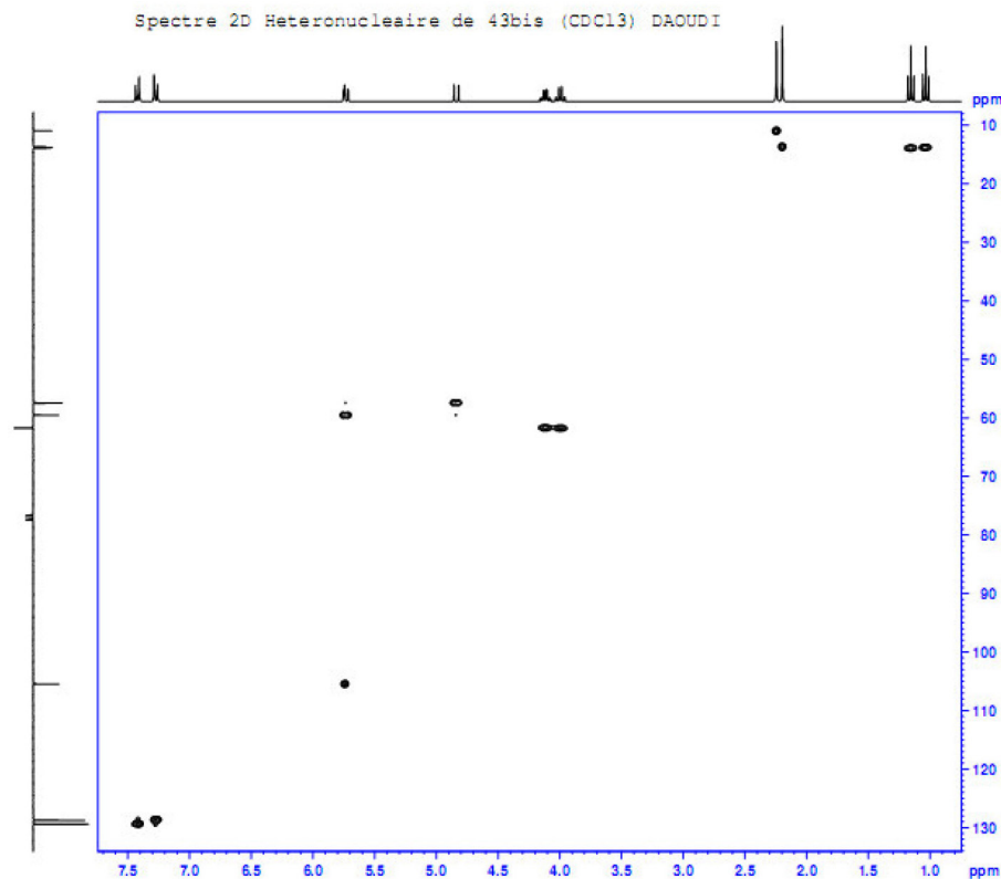
Figure S18. HETCOSY of compound 10 in CDCl 3 .
