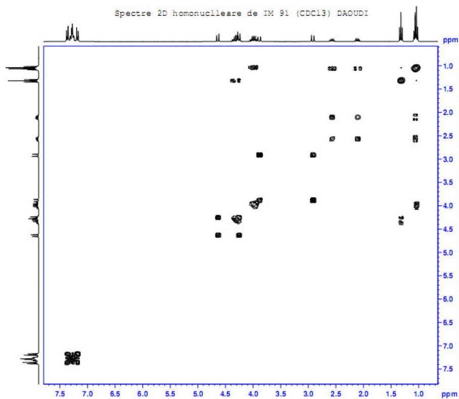
Figure S25. COSY of compound 12 in CDCl 3 .
