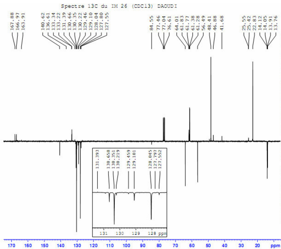
Figure S12. 13 C NMR (75.5 MHz) spectrum of compound 9 in CDCl 3 .
