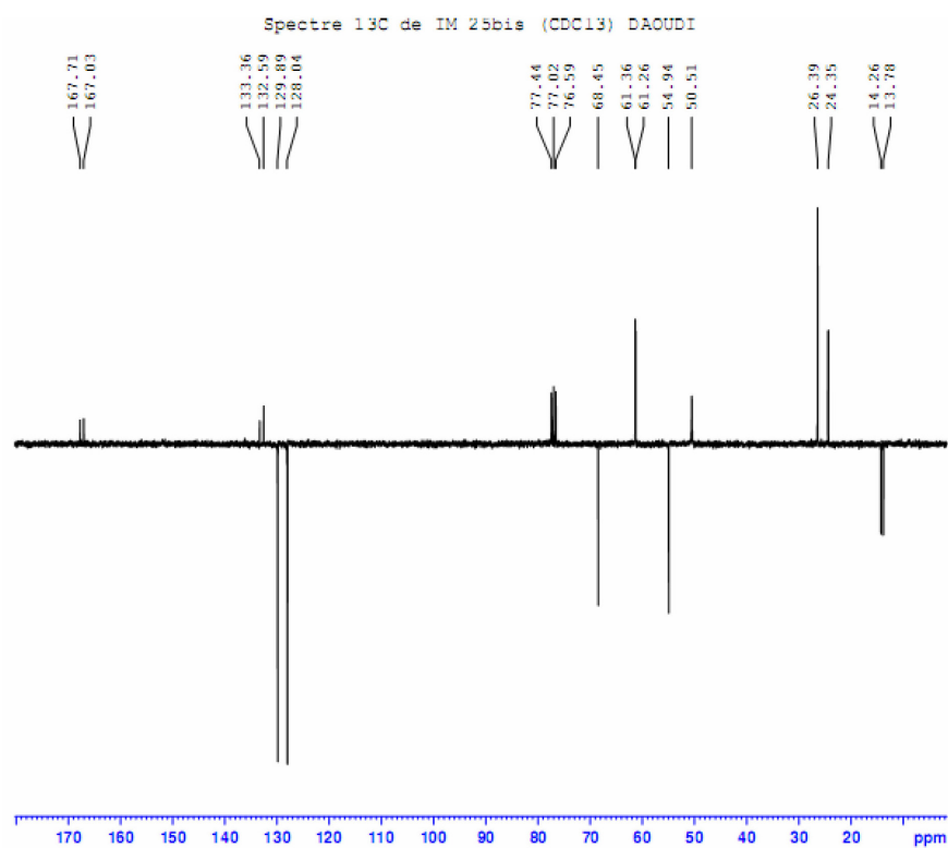
Figure S20. ^{13}\text{C} NMR (75.5 MHz) spectrum of compound 11 in \text{CDCl}_3 .
