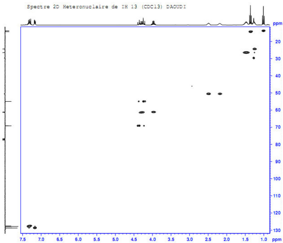
Figure S4. HETCOR of compound 6 in CDCl 3 .
