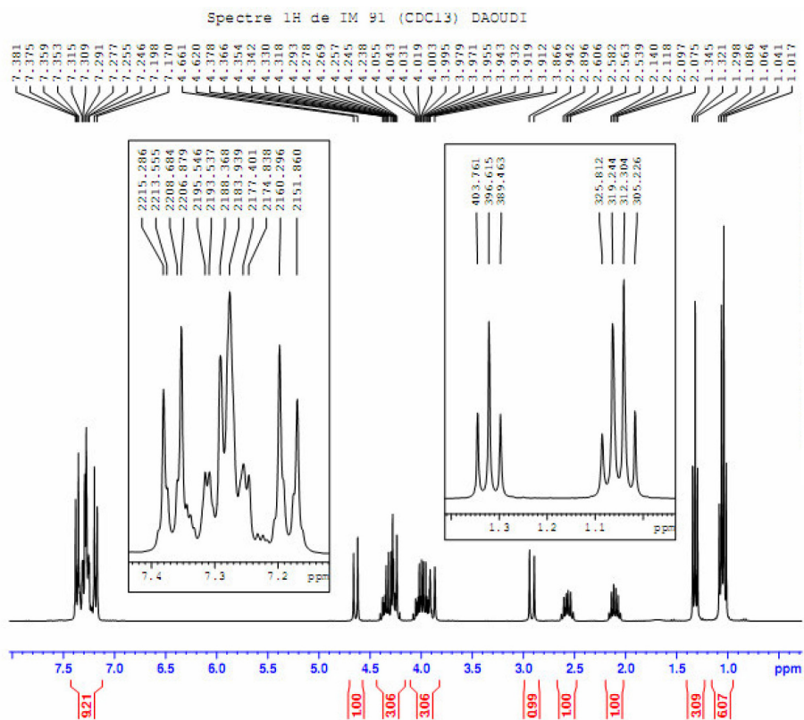
Figure S23. 1 H NMR (300 MHz) spectrum of compound 12 in CDCl 3 .
