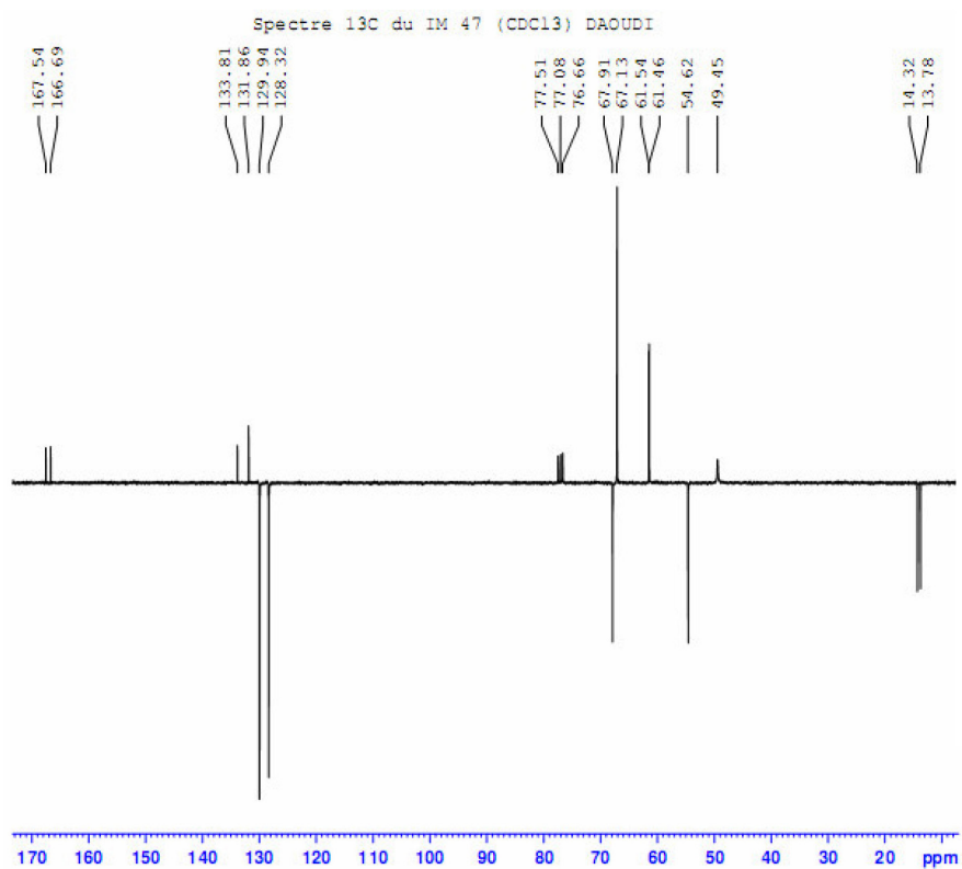
Figure S7. 13 C NMR (75 MHz) spectrum of compound 7 in CDCl 3 .
