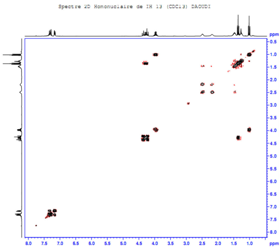
Figure S5. COSY of compound 6 in CDCl 3 .
