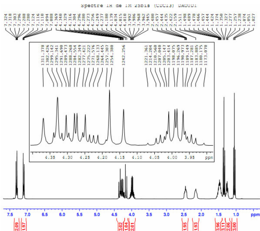
Figure S19. 1 H NMR (300 MHz) spectrum of compound 11 in CDCl 3 .
