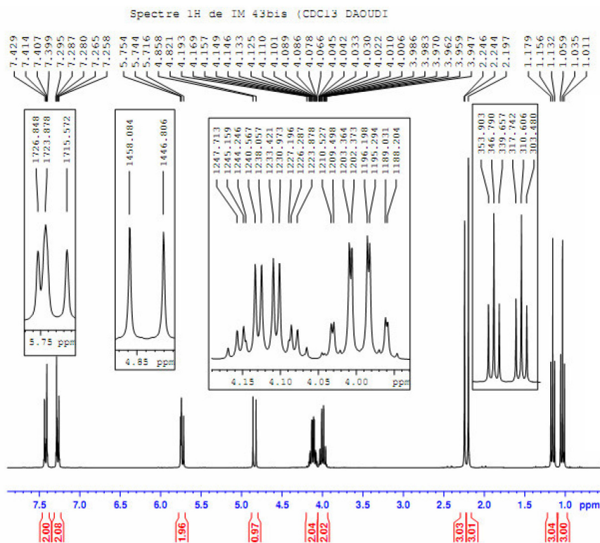
Figure S15. 1 H NMR (300 MHz) spectrum of compound 10 in CDCl 3 .
