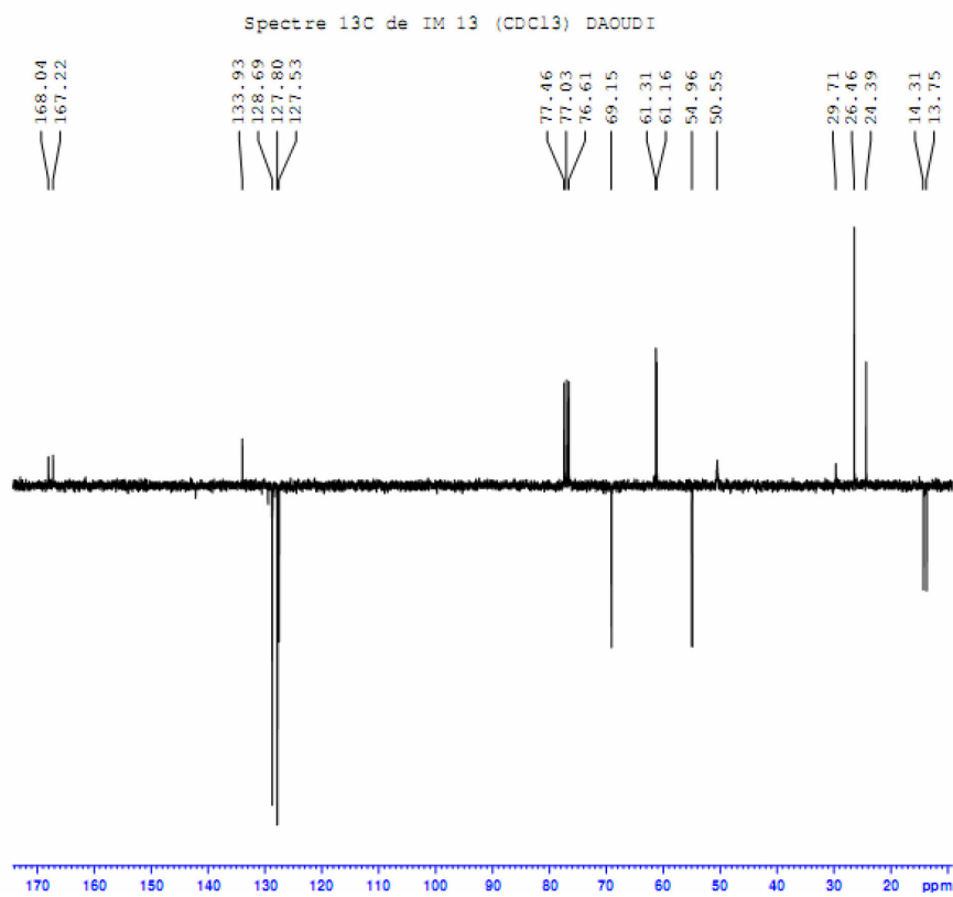
Figure S3. ^{13}\text{C} NMR (75 MHz) spectrum of compound 6 in \text{CDCl}_3 .
