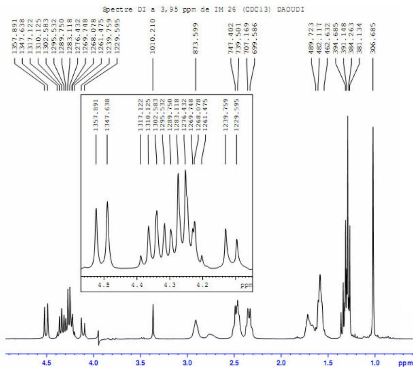
Figure S14. 1 H NMR (300 MHz) spectrum of compound 9 in CDCl 3 expanded at 4.5-1.0 ppm.
