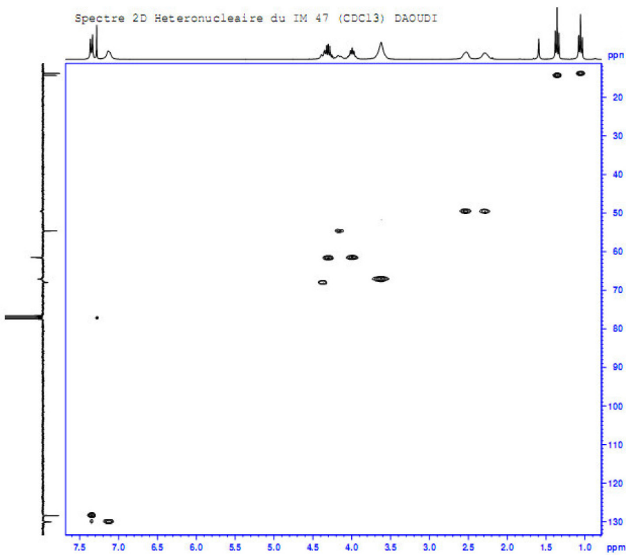
Figure S9. HETCOSY of compound 7 in CDCl 3 .
