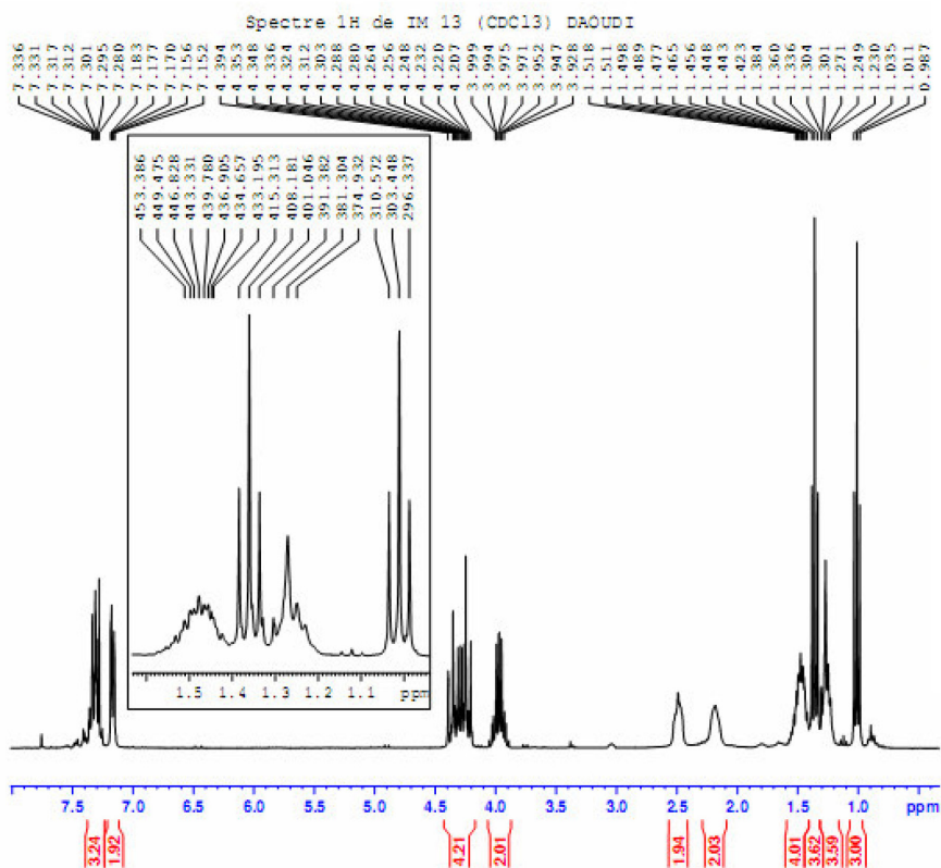
Figure S1. 1 H NMR (300 MHz) spectrum of compound 6 in CDCl 3 .
