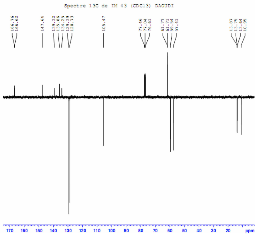
Figure S16. 13 C NMR (75.5 MHz) spectrum of compound 10 in CDCl 3 .
