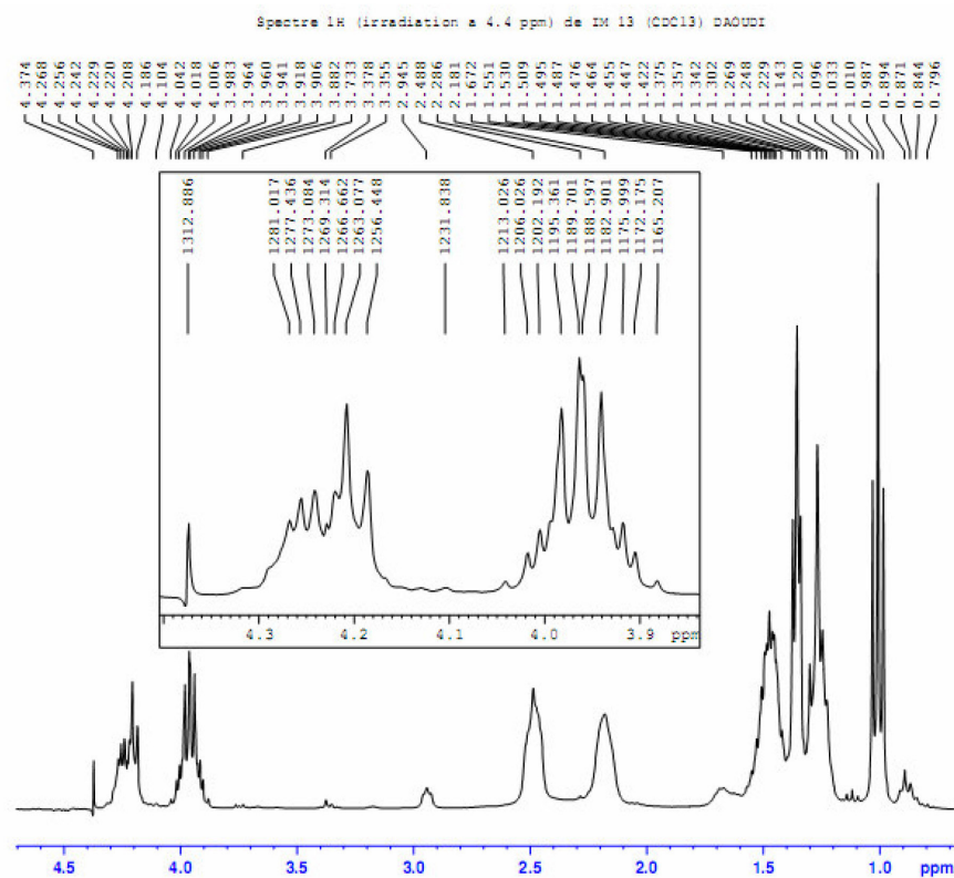
Figure S2. ^1\text{H} NMR (300 MHz) spectrum of compound 6 in \text{CDCl}_3 expanded at 4.5-1.0ppm.
