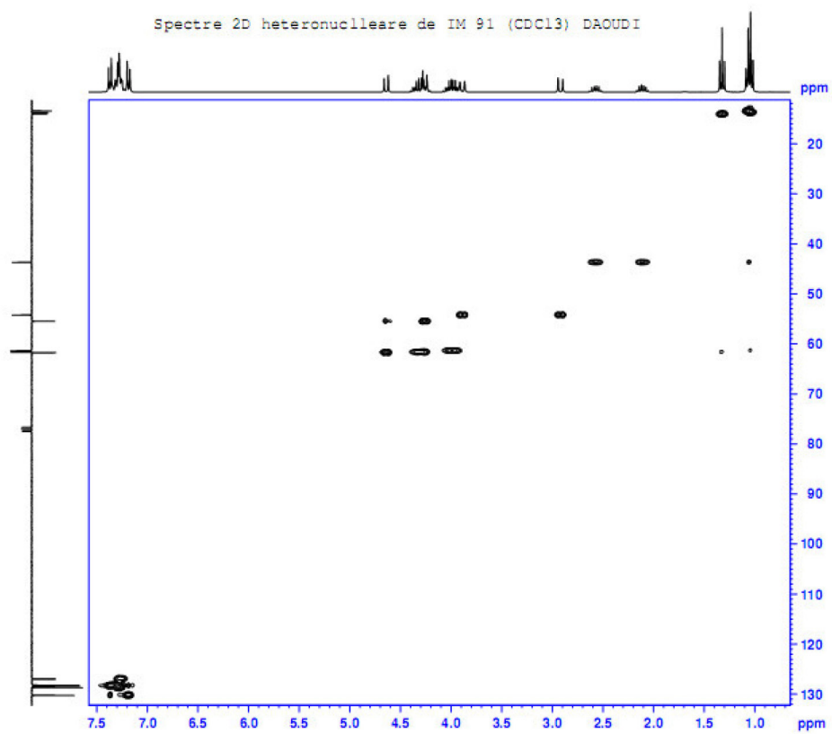
Figure S26. COSY of compound 12 in CDCl 3 .
