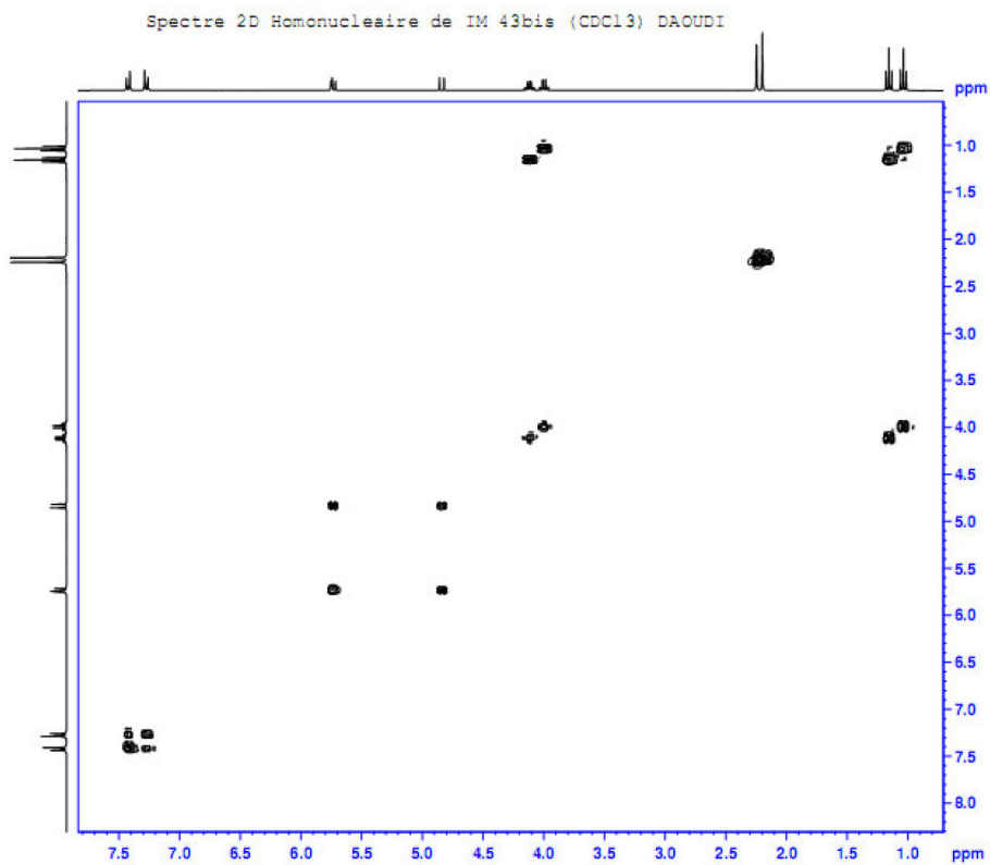
Figure S17. COSY of compound 10 in CDCl 3 .
