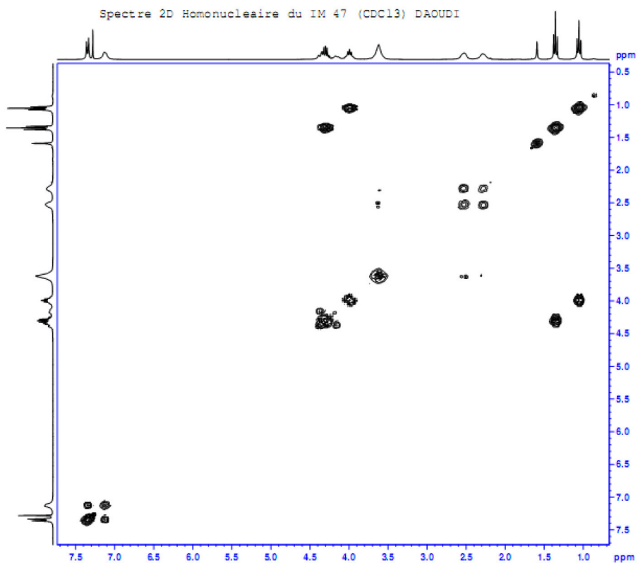
Figure S8. COSY of compound 7 in CDCl 3 .
