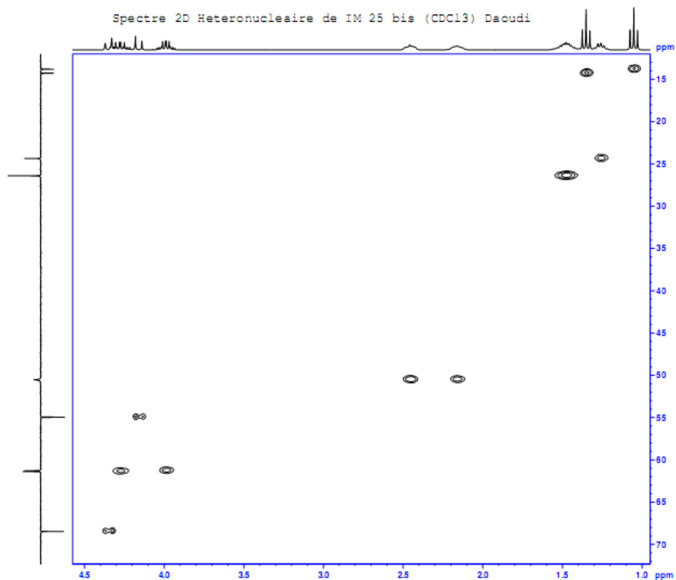
Figure S22. HETCOSY of compound 11 in CDCl 3 .
