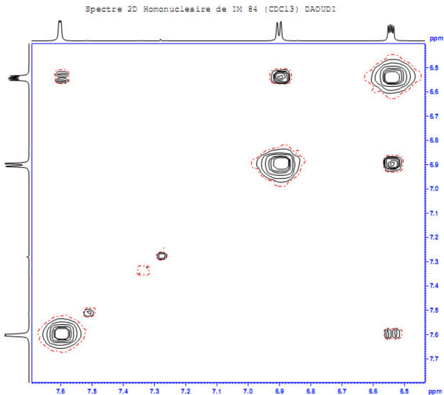
Figure S10. COSY of compound 7 in CDCl 3 .
