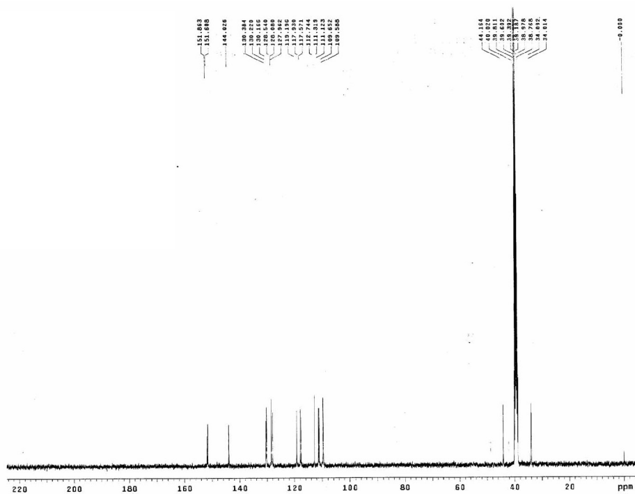
Figure S14. 13 C NMR spectrum of 3c.
