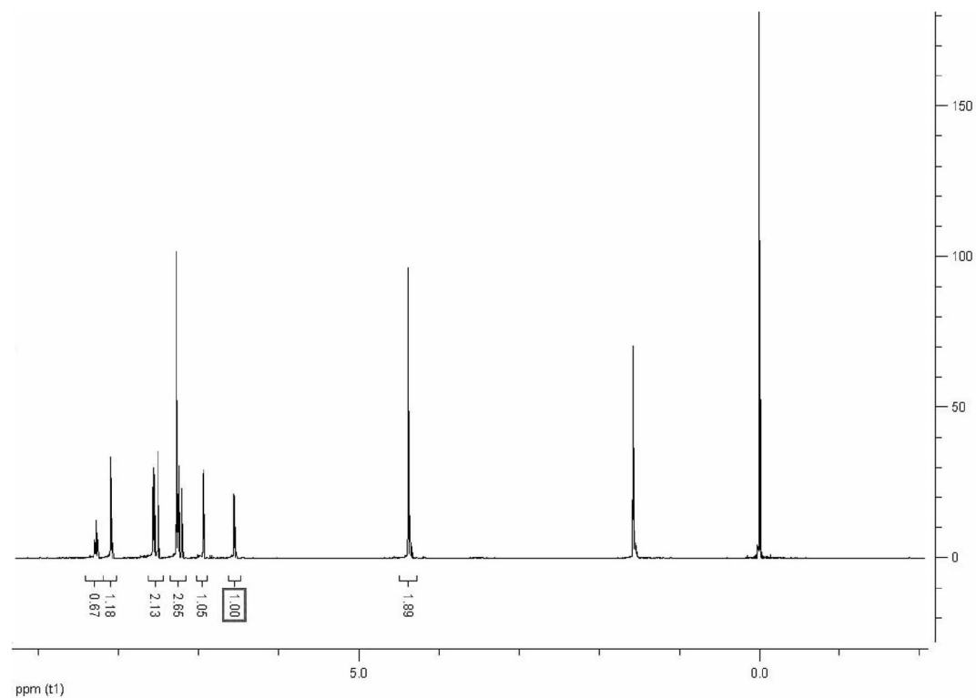
Figure S22. 1 H NMR spectrum of 3f .
