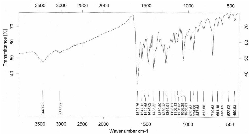
Figure S15. IR spectrum of 3c.
