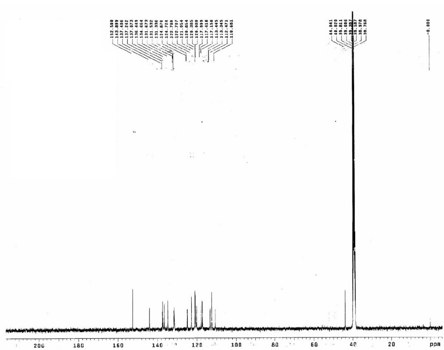
Figure S11. 13 C NMR spectrum of 3b.
