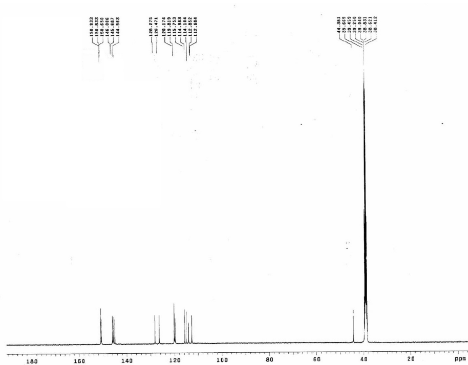
Figure S20. ^{13}\text{C} NMR spectrum of 3e .
