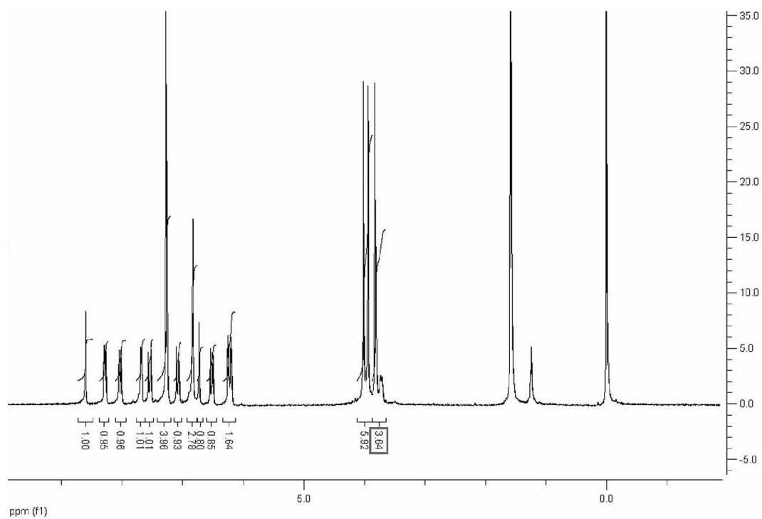
Figure S13. 1 H NMR spectrum of 3c.
