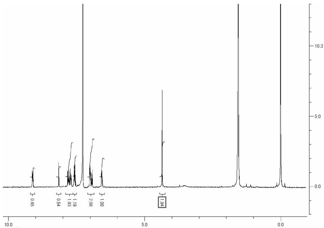
Figure S19. ^1\text{H} NMR spectrum of 3e.
